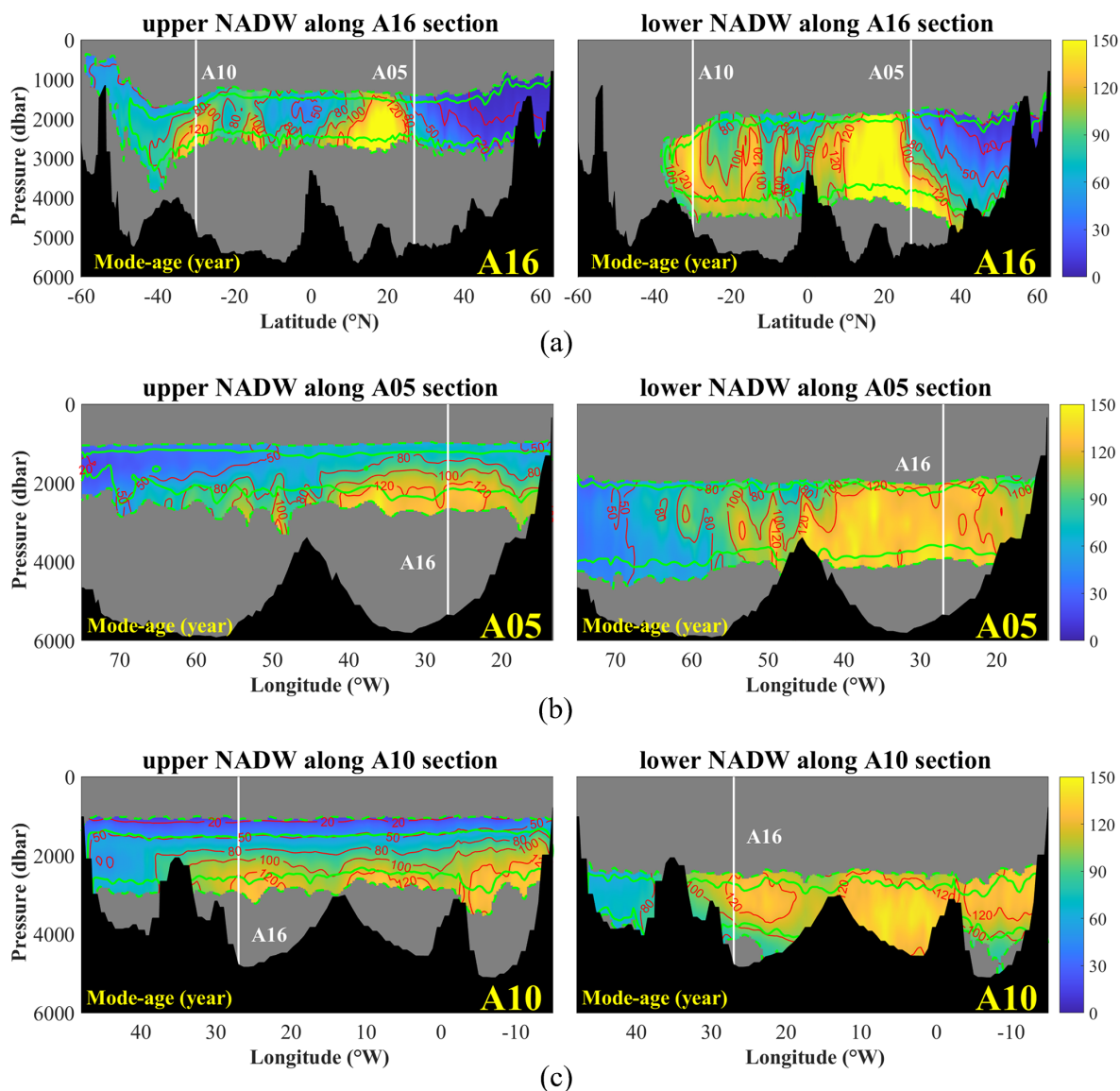
Figure 11. Mode-ages (years) of upper and lower NADW along the A16 (a), A05 (b) and A10 (c) section lines. The green contour lines show fractions of water masses in 50 % and the dashed green lines show the 20 % fractions. The grey blank indicates less than 20 % contribution from NADW. The white vertical lines show cross overs with other section lines.
