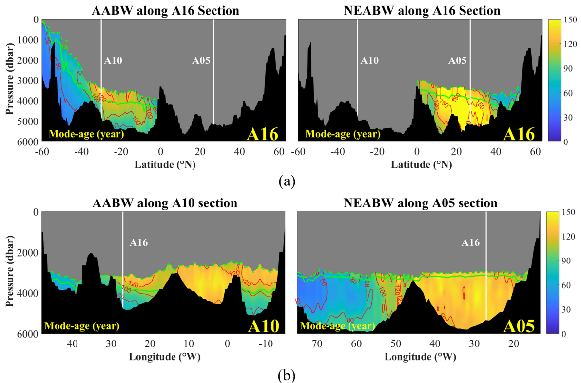
Figure 13. Mode-ages of AABW and NEABW along the A16 (a), A05 and A10 (b) section lines. The green contour lines show fractions of water masses in 50 and the dashed green lines show the 20 % fractions. The grey blank indicates less than 20 % contribution from bottom water masses. The white vertical lines show cross overs with other section lines.
