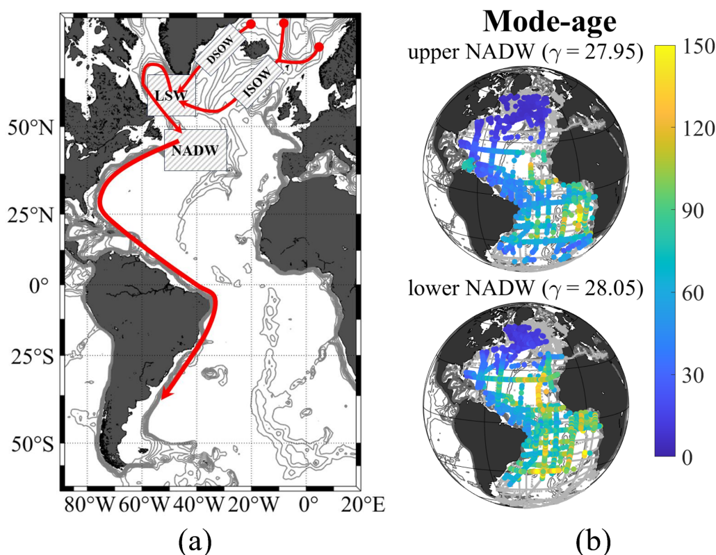
Figure 10. Mode-ages of upper and lower NADW in the Atlantic Ocean. (a) Main currents in the deep and overflow layer. The currents (arrows) and the formation areas (rectangular shadows) of water masses in the deep and overflow layer. (b) The mode-ages (years) of upper and lower NADW at their core neutral densities ( \text{kg m}^{-3} ). The colored dots show the ages in each station. The grey dots show all the GLODAPv2 stations that have less than 20 % contribution of the water mass in question or lack of transient-tracer data.
