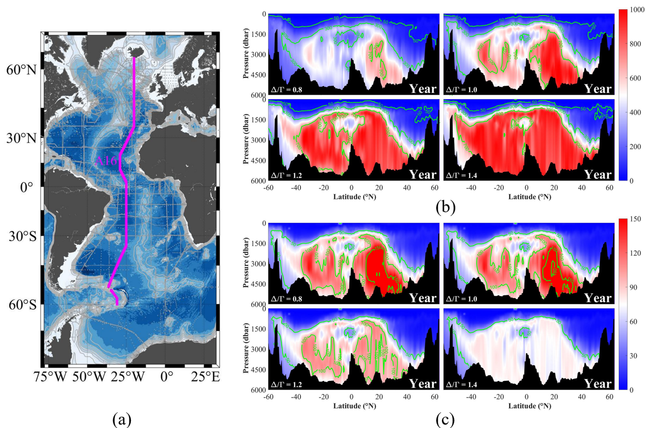
Figure 3. (a) Map of the A16 section under the framework of the WOCE/GO-SHIP project in 2013. (b) Distributions of mean-ages and (c) mode-ages under varying mixing ratios ( \Delta/\Gamma = 0.8, 1.0, 1.2 , and 1.4 ) derived from GLODAPv2 observational data. Green contour lines correspond to mean-ages of 50, 300, and 700 years and mode-ages of 50, 100, and 150 years, respectively.
