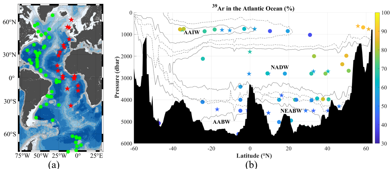
Figure 16. (a) Map of the ^{39}\text{Ar} sampling stations. The green circle dots show the stations in the west Atlantic Ocean (west of the Mid Atlantic Ridge), while the red stars show the stations in the east Atlantic Ocean. (b) Distributions of ^{39}\text{Ar} in the Atlantic Ocean (% Modern). The circle dots show the data in the west, while the stars show the data in the east Atlantic Ocean. The solid isolines show the 80 % fractions of water masses and the dashed lines show the 50 % fractions.
