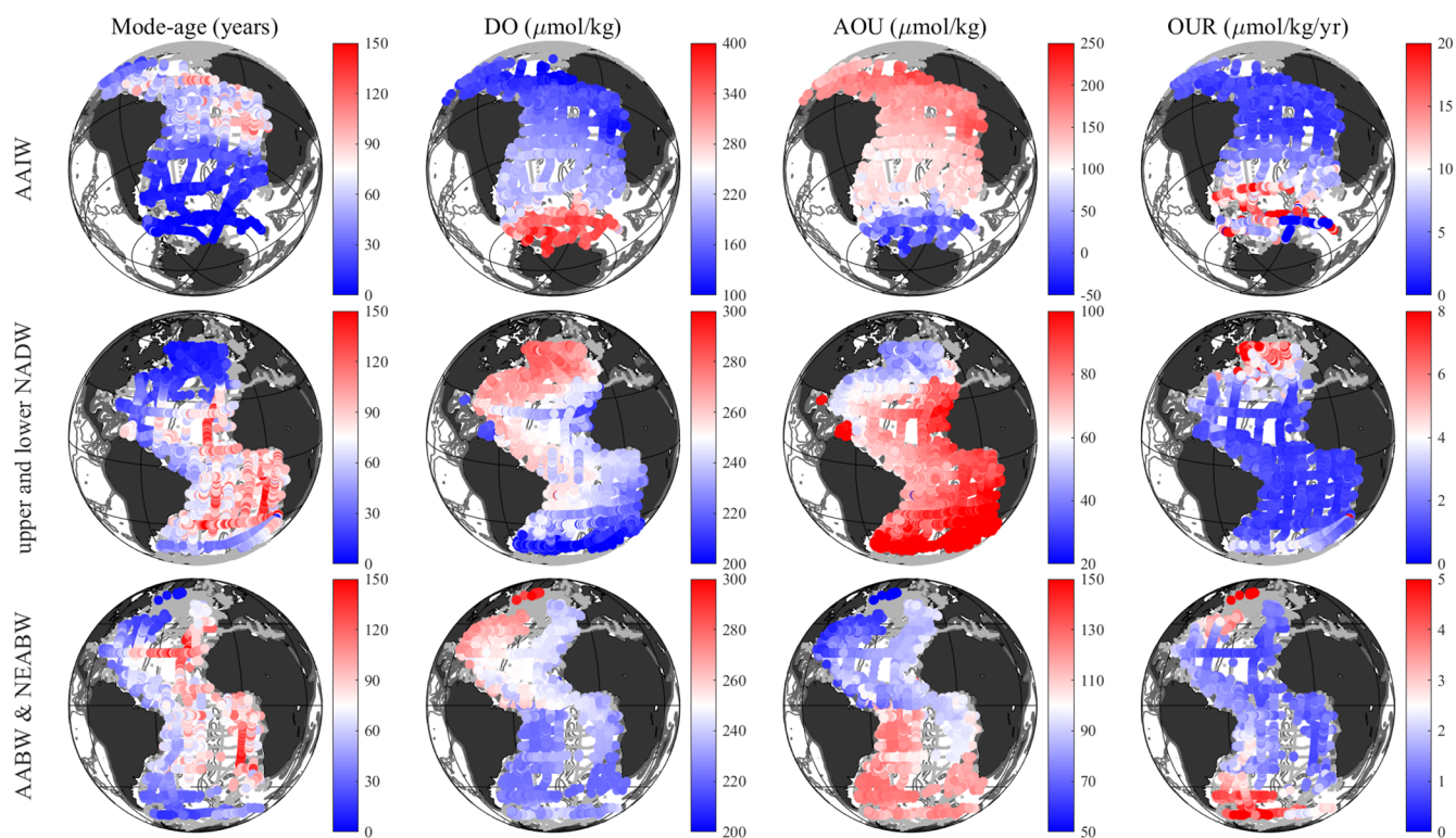
Figure 14. Mode-age, DO, AOU and OUR of wide-spread water masses in the Atlantic Ocean. The colored dots show the values in each station at core neutral densities of each water mass (AAIW at 27.20, upper NADW at 27.95, lower NADW at 28.05, AABW at 28.15, NEABW at 28.10 kg m -3 ), the upper and lower NADW, AABW and NEABW are shown in one plot. The grey dots show all the GLODAPv2 stations that have less than 20 % contribution of the water mass in question. Note: Negative AOU values indicate oxygen supersaturation, which is typically observed in well-ventilated surface or near-surface waters.
