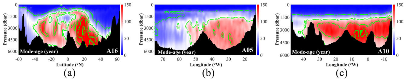
Figure 5. Mode-ages along the three selected WOCE/GO-SHIP sections.
