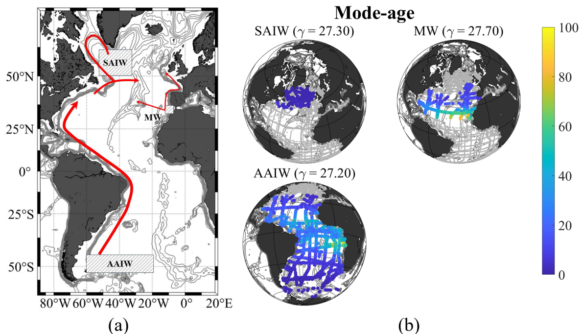
Figure 8. Mode-ages of intermediate water masses in the Atlantic Ocean. (a) Main currents in the intermediate layer. The currents (arrows) and the formation areas (rectangular shadows) of water masses in the intermediate layer. (b) The mode-ages of intermediate water masses at their core neutral densities ( \text{kg m}^{-3} ). The colored dots show the ages in each station. The grey dots show all the GLODAPv2 stations that have less than 20% contribution of the water mass in question or lack of transient-tracer data.
