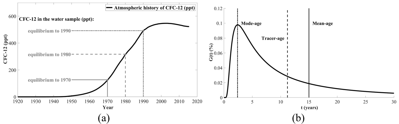
Figure 1. Schematic diagram illustrating three concepts of water mass ages. (a) The tracer age: The transient tracer (such as CFC-12) in the water sample in equilibrium with the atmospheric at a certain year. This approach assumes that the ocean is a purely advective process (without mixing); (b) The concepts of mean- and mode-ages: Based on the inverse Gaussian transport time distribution model, assuming the mixing ratio ( \Delta/\Gamma = 1 ) and observed tracer partial pressure CFC-12 = 300 ppt, as an example. Shown are the positions of the mean-age ( \Gamma ), tracer age, and the mode-age ( \tau_{\text{mode}} ).
