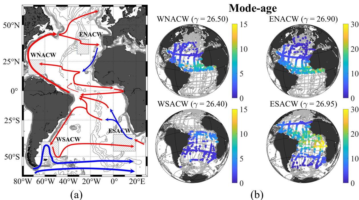
Figure 6. Mode-ages of central water masses in the Atlantic Ocean. (a) The main currents in the upper layer with warm (red) and cold (blue) currents and the approximate formation areas (rectangular shadows) of central water masses. (b) Mode-ages of central water masses at their core neutral densities ( \text{kg m}^{-3} ). The colored dots show the ages in each station. The grey dots show all the GLODAPv2 stations that have less than 20 % contribution of the water mass in question or lack of transient-tracer data.
