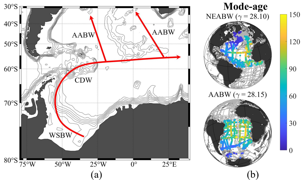
Figure 12. Mode-ages of bottom water masses in the Atlantic Ocean. (a) Main currents in the bottom layer. The currents (arrows) and the formation areas (rectangular shadows) of water masses in the deep and overflow layer. (b) The mode-ages (years) of bottom water masses at their core neutral densities ( \text{kg m}^{-3} ). The colored dots show the ages in each station. The grey dots show all the GLODAPv2 stations that have less than 20 % contribution of the water mass in question or lack of transient-tracer data.
