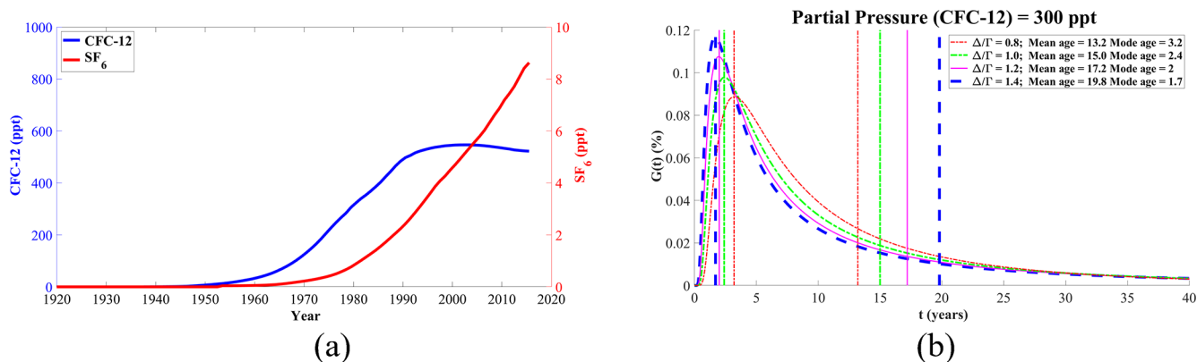
Figure 2. The relationships between mean-age, mode-age and mixing ratio ( \Delta/\Gamma ). (a) Historical atmospheric partial pressure data of transient tracers over time (CFC-12 and SF 6 ) in the Northern Hemisphere (data source: Bullister et al., 2002); (b) Relationship between mean-ages and mode-ages under same partial pressure (CFC-12 = 300 ppt) but different mixing ratios ( \Delta/\Gamma ) assuming the sampling year is 1990.
