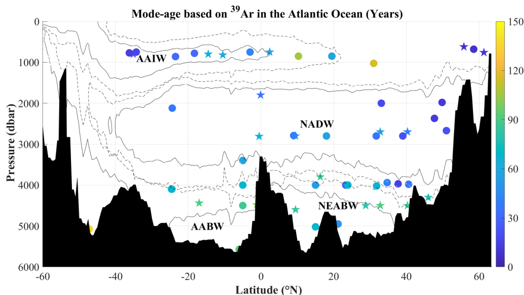
Figure 17. Mode-ages of the wide-spread water masses estimated by ^{39}\text{Ar} in the Atlantic Ocean. The circle dots show the data in the west, while the stars show the data in the east Atlantic Ocean. The solid isolines show the 80 % fractions of water masses and the dashed lines show the 50 % fractions.
