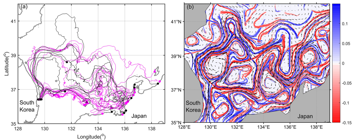
Figure 2. (a) Observed trajectories of undrogued DX drifters (black lines) and drogued DO drifters (magenta lines). Thick black lines indicate the initial deployment locations, and filled circles denote the final positions of drifters that remained at sea. (b) Signed Finite-time Lyapunov exponent (FTLE) field computed from the geostrophic velocity averaged over the first week after drifter release. Black arrows indicate the geostrophic velocity vectors. In the signed FTLE representation, blue and red ridges indicate repelling and attracting Lagrangian structures, respectively.
