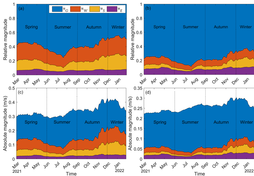
Figure 12. The relative and absolute value of the current components at the surface (a, c) and 1.5 m depth (b, d) of ( u_G – geostrophic current, u_W – wind-driver current, u_S – Stoke current and u_E – Ekman current) from March 2021 to February 2022.
