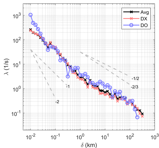
Figure 4. Finite-Size Lyapunov Exponent (FSLE), \lambda , as a function of separation distance, \delta , for the observed drifters. The black line represents the average of all drifters, the red line represents the undrogued (DX) drifters, and the blue line represents the drogued (DO) drifters. The dashed gray lines indicate reference slopes of -2 , -1 , -1/2 , and -2/3 .
