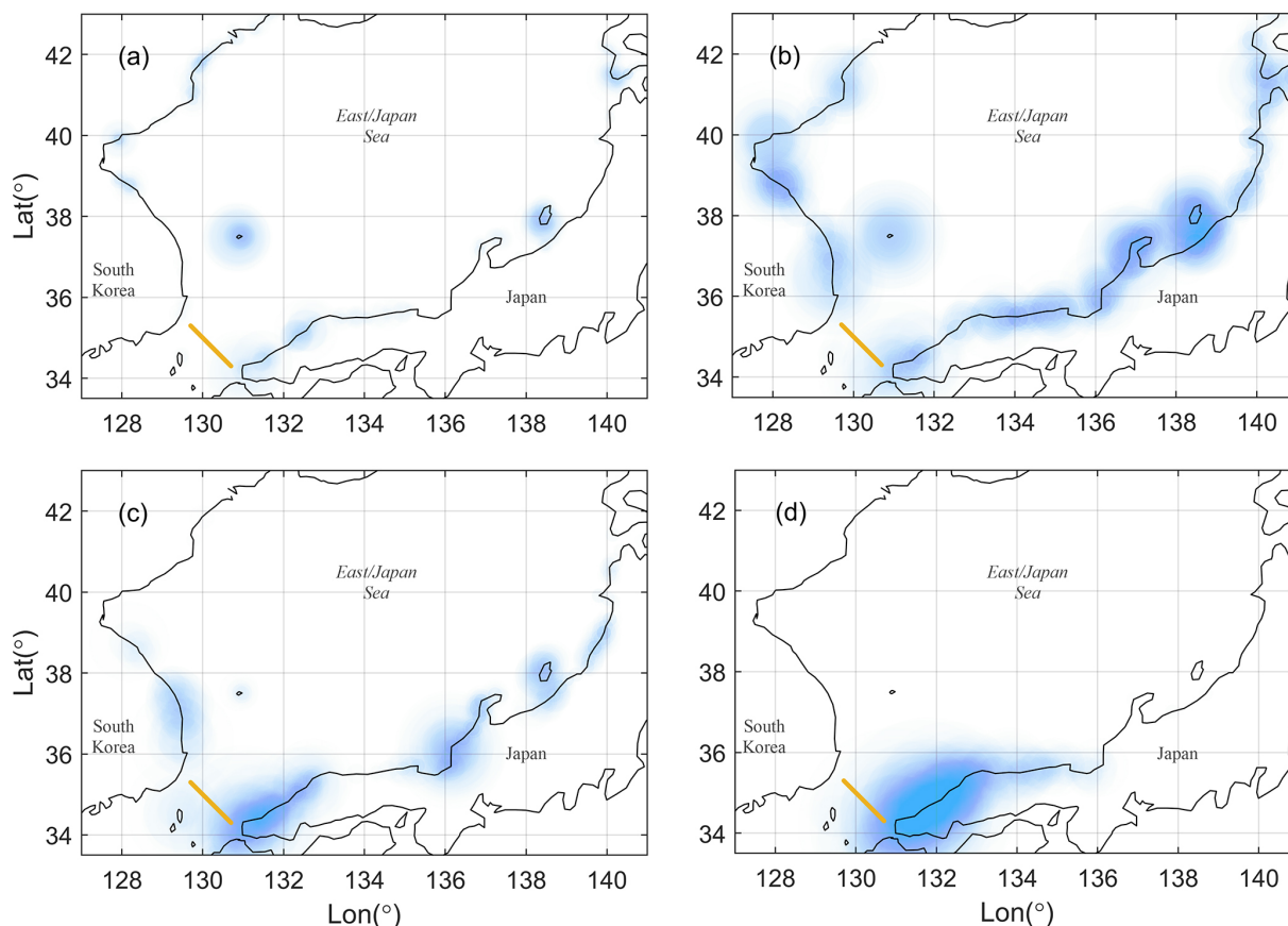
Figure 14. Spatial distribution and relative accumulation intensity of beached particles simulated using the optimal surface forcing (C7) for (a) spring (March–May), (b) summer (June–August), (c) fall (September–November), and (d) winter (December–February). The beached particle locations were determined from the same particle trajectories used in Fig. 13. Beaching is defined as the behavior of particles first contacting the coastline. The particle release location is marked by the yellow line. Color intensity along the coastline indicates the relative density of particle accumulation, with darker shades representing higher accumulation.
