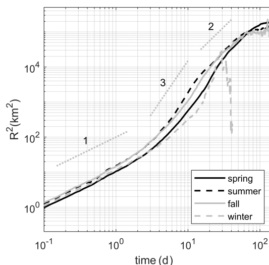
Figure 15. Seasonal variation of relative dispersion, R^2(t) , for particles (same as those used in Figs. 13 and 14) simulated using the optimal forcing combination (C7). Lines indicate relative dispersion for particles released in spring (black solid), summer (black dashed), autumn (gray solid), and winter (gray dashed).
