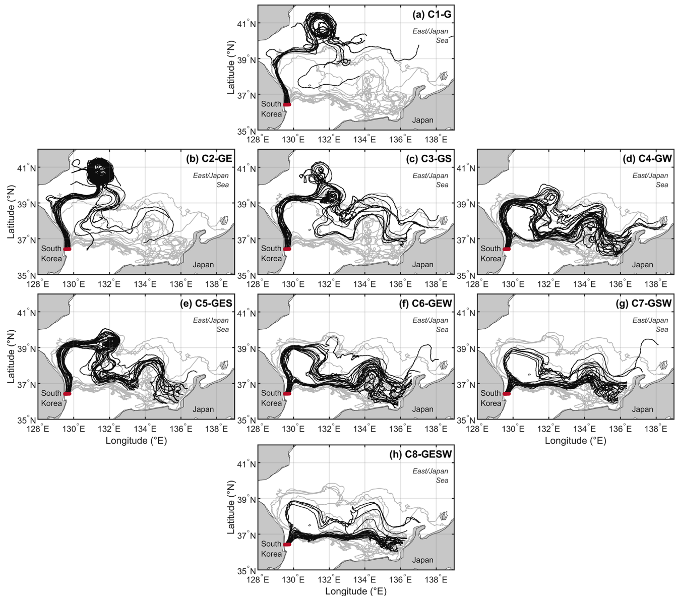
Figure 5. Observed trajectories of undrogued DX drifters (gray) and simulated PTM-DX trajectories (black) over the 79 d simulation period for forcing combinations C1–C8 listed in Table 1. Red markers indicate the initial release locations. All panels use the same geographic domain, coordinate units, and labels for South Korea, Japan, and the East/Japan Sea. Panels (a)–(h) correspond to C1–C8 and are arranged by the number of forcing components: C1; C2–C4; C5–C7; and C8. G , E , S , and W denote geostrophic current, Ekman current, Stokes drift, and windage, respectively.
