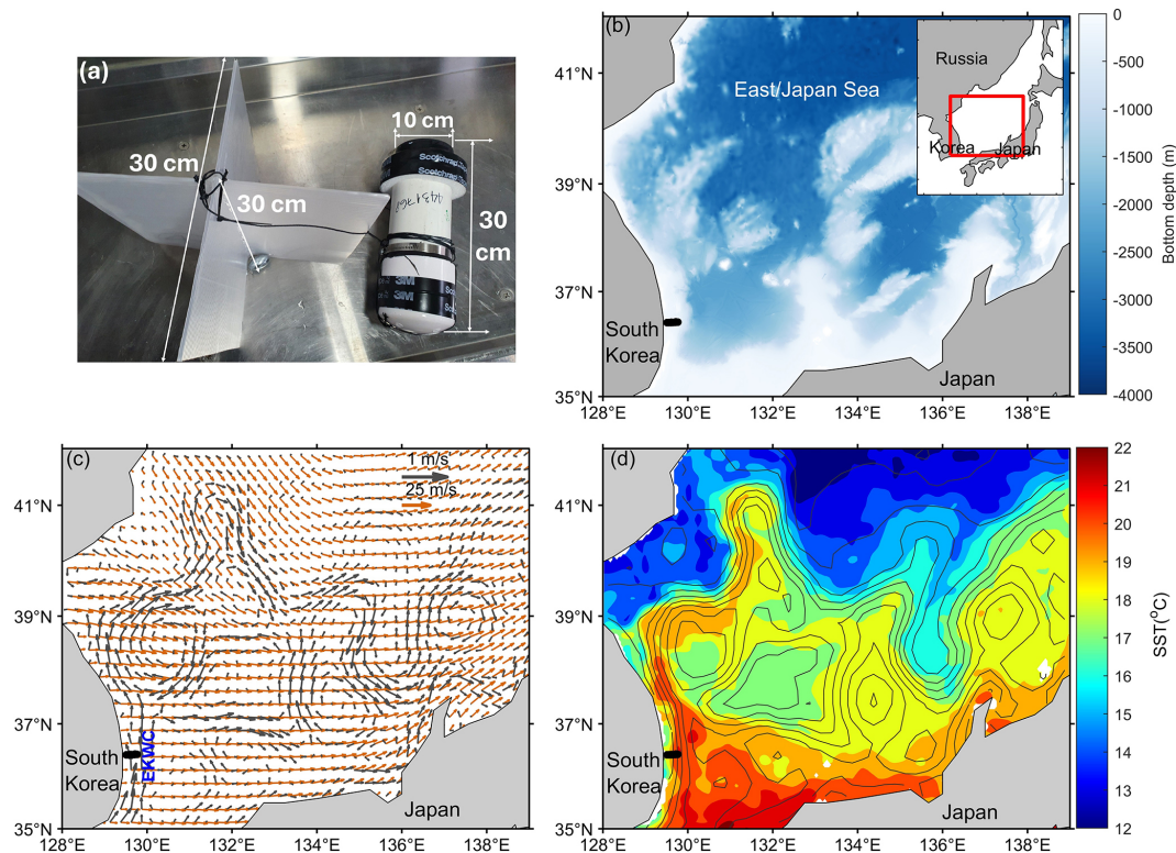
Figure 1. (a) Photograph and dimensions of the undrogued DX and drogued DO drifters. (b) Bathymetry of the East/Japan Sea, with the inset showing the surrounding geographic region. (c) Geostrophic current vectors (black) and 10 m wind velocity vectors (orange), both averaged over the first week after drifter release. The East Korea Warm Current (EKWC) is indicated in blue, and the reference vectors are shown in the upper-right corner. (d) Sea surface temperature (SST; color shading) and sea surface height (SSH; contour lines), both averaged over the first week after drifter release. Thick black lines indicate the initial drifter deployment locations.
