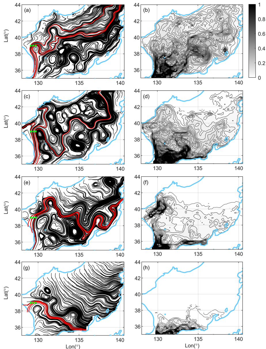
Figure 13. Seasonal streamlines and particle accumulation maps from March 2021 to February 2022, simulated using the optimal forcing combination (C7). Panels (a), (c), (e) and (g) show streamlines of the seasonally averaged surface current for spring (March–May), summer (June–August), autumn (September–November), and winter (December–February), respectively. Panels (b), (d), (f) and (h) show the corresponding seasonal particle accumulation maps. Red lines represent streamlines that pass through three fixed points marked in green. Particles were released every five days from March 2021 to February 2022 at the southwestern entrance of the EJS and tracked for five months. The accumulation maps display the relative frequency of particle occurrence, calculated as the number of particle passages through each 5 km grid cell normalized by the maximum frequency.
