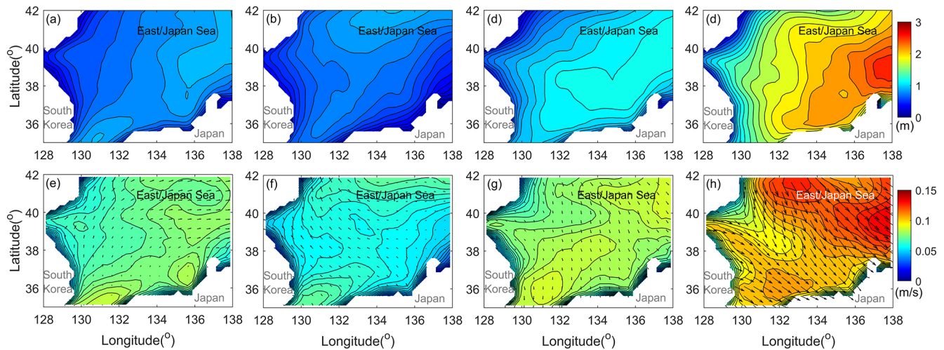
Figure 11. The mean of significant wave height (a–d), wind (e, f) in EJS for each season in 2021: (a, e) spring (1 March–30 May), (b, f) summer (1 June–30 August), (c, g) autumn (1 September–30 November), and (d, h) winter (1 December–28 February).
