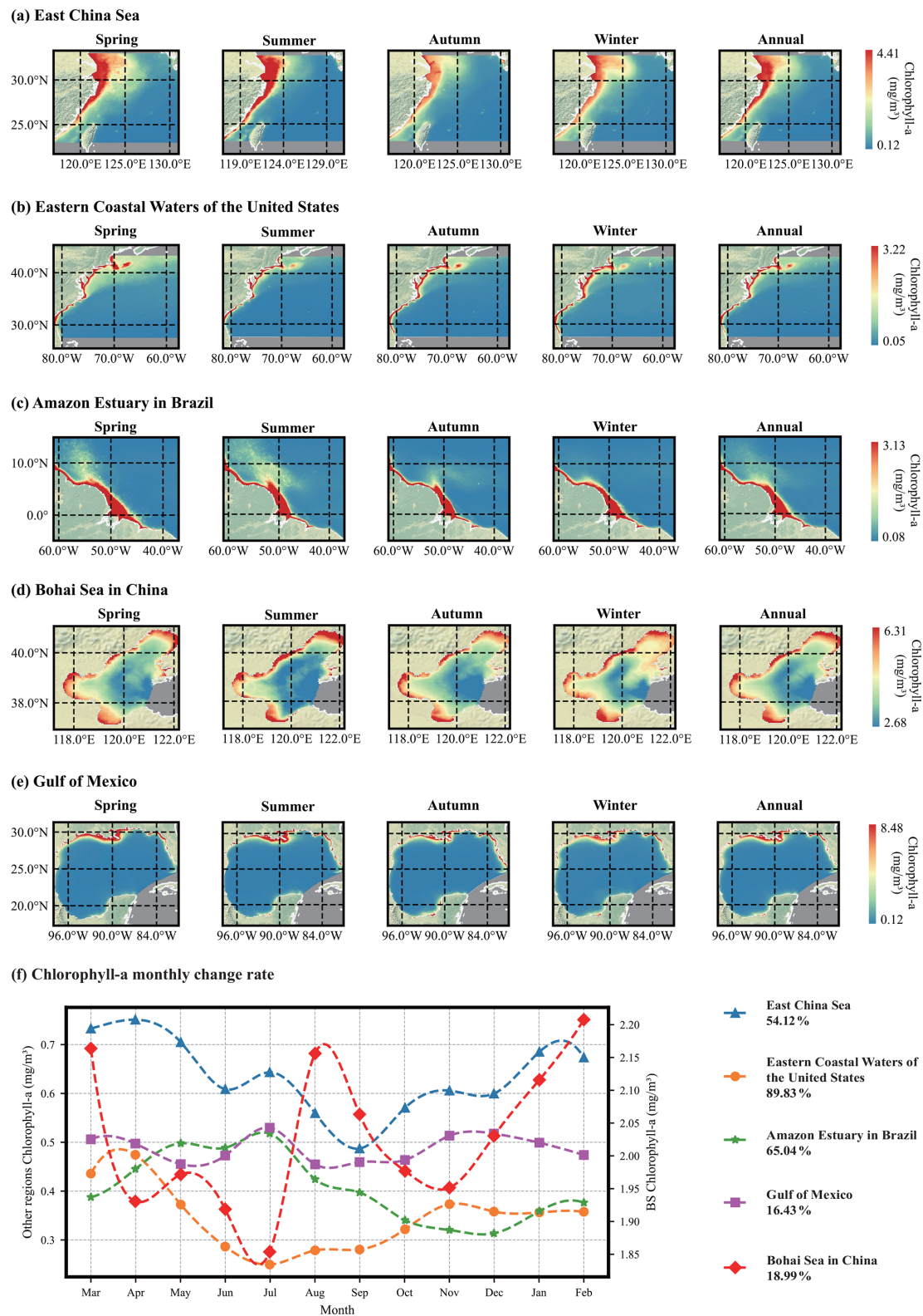
Figure 4. Spatial distribution of annual and seasonal Chl a concentrations at the five sites: (a) the East China Sea, (b) the Eastern Coastal Waters of the United States, (c) the Amazon Estuary, (d) the Bohai Sea, and (e) the Gulf of Mexico. (f) Monthly variation of Chl a concentrations. The Bohai Sea is shown on the right y-axis, whereas the other four seas are shown on the left y-axis. The data on the right are the monthly change rates. Areas shown in light gray-blue indicate missing data.
