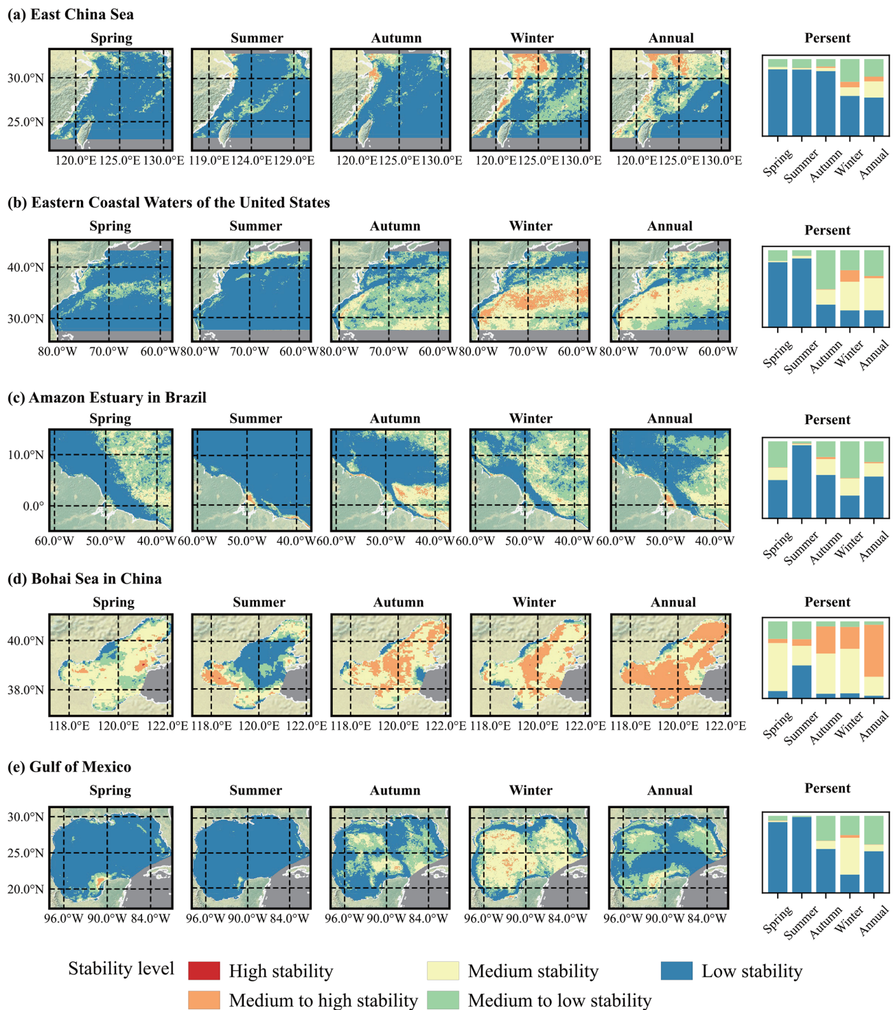
Figure 7. The spatial distribution of the coefficient of variation of seasonal and annual Chl a from 1998 to 2020 in (a) the East China Sea, (b) the Eastern Coastal Waters of the United States, (c) the Amazon Estuary, (d) the Bohai Sea, and (e) the Gulf of Mexico. The percentage bar chart shows the proportion of areas with different stabilities during each season.
