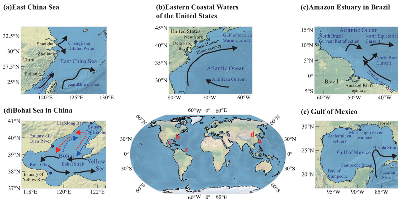
Figure 1. The geographic locations and major current systems of the five studied sea areas: (a) the East China Sea located in the range of 117–131° E and 23–33° N; (b) the Eastern Coastal Waters of the United States located in the range of 81.6–57.66° W and 27.5–43.3° N; (c) the Amazon Estuary located in the range of 16° N–6° S and 61–37° W; (d) the Bohai Sea located in the range of 37–41° N and 117–123° E; and (e) the Gulf of Mexico located in the range of 17.09–31.16° N and 98.86–81.28° W. Note: The base maps for the land and ocean portions of the map artifacts are land-cover data and ocean polygon data (rendered in gray) and are available for download from Natural Earth ( https://www.naturalearthdata.com , last access: 25 May 2026).
