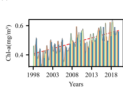
(e) Gulf of Mexico
