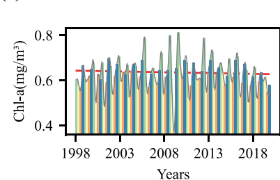
(a)East China Sea
