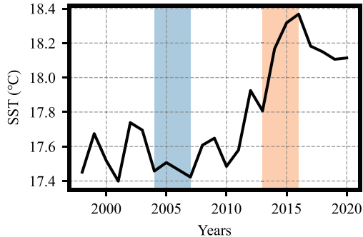
(e) Gulf of Mexico
