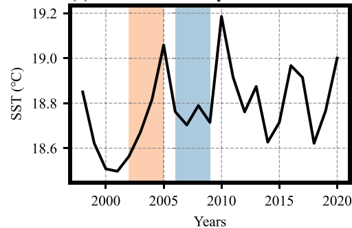
(c) Amazon Estuary in Brazil
