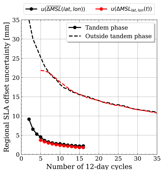
Figure 6. Comparison of two uncertainty estimation methods for J3/S6A in a regional analysis using a 3 \times 3^\circ grid resolution.
