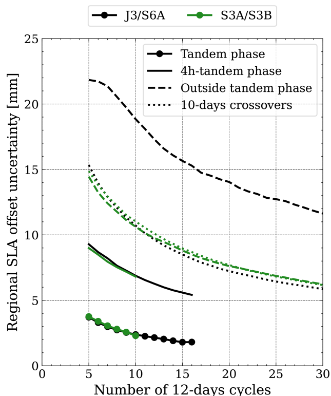
Figure 4. J3/S6A (black) and S3A/S3B (green) regional SLA offset uncertainties on 3 \times 3^\circ grid for 12 d subcycles. Uncertainties are computed using the temporal method for four different comparison configurations: tandem phase, 4 h tandem phase, outside tandem phase and 10 d dual-crossovers.
