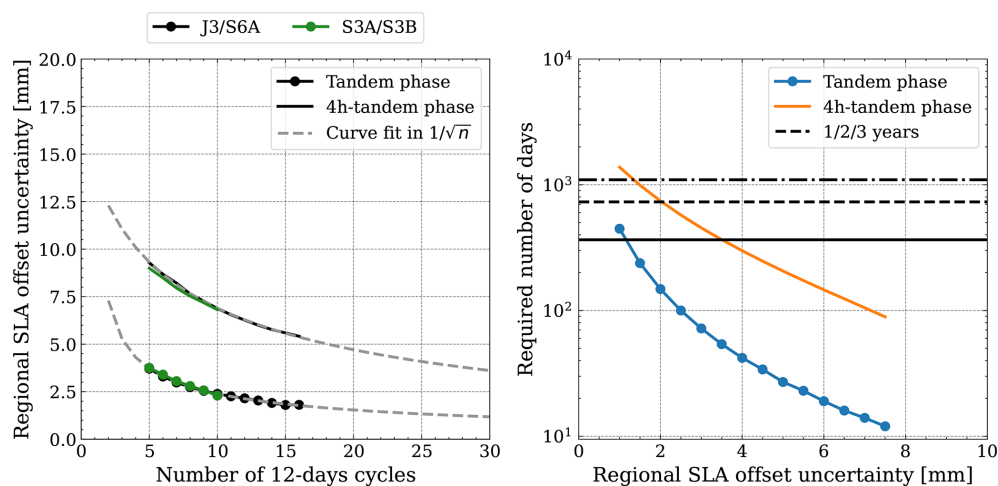
Figure 5. Use of the J3/S6A comparison during the tandem phase to fit the uncertainty evolution (left figure) and to estimate the number of days (right figure) required for the 4 h tandem phase (orange) to reach the same precision as the classical tandem phase (blue). The horizontal black lines indicate, from bottom to top, the 1-, 2-, and 3-year thresholds.
