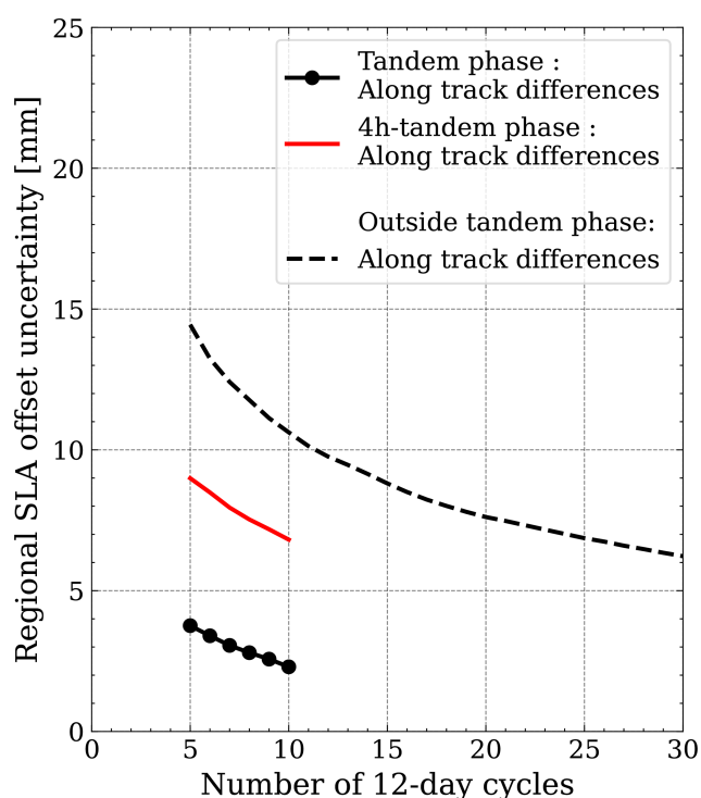
Figure 2. S3A and S3B regional SLA offset uncertainties on 3 \times 3^\circ grid for 12 d subcycles. Uncertainties are computed using the temporal method for three different configurations: classical tandem phase, 4 h tandem phase, and outside tandem phase.
