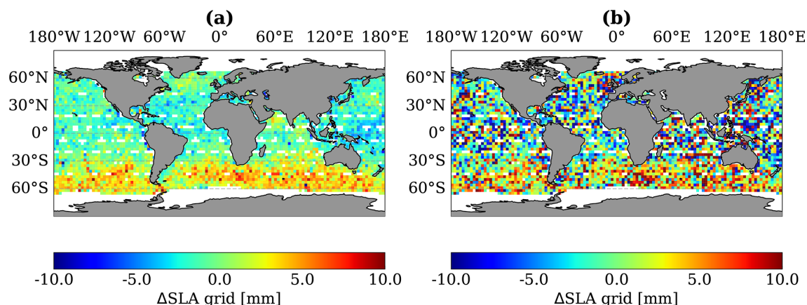
Figure 3. Differences between S3A and S3B for (a) classical tandem phase for 3 \times 3^\circ boxes and (b) 4 h tandem phase for 3 \times 3^\circ boxes.
