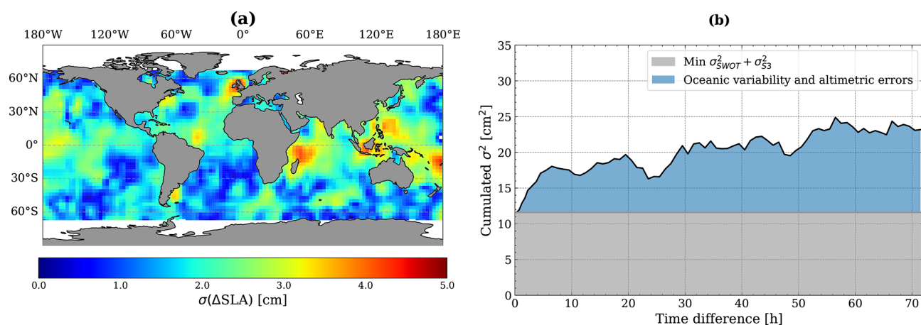
Figure 1. (a) Map of variability in 4 h time interval, from SWOT KaRIn and S3A and S3B dual-crossovers and (b) time series of the cumulated variance of \Delta\text{SLA} ; decomposition between instrumental errors (grey) and oceanic variability (blue).
