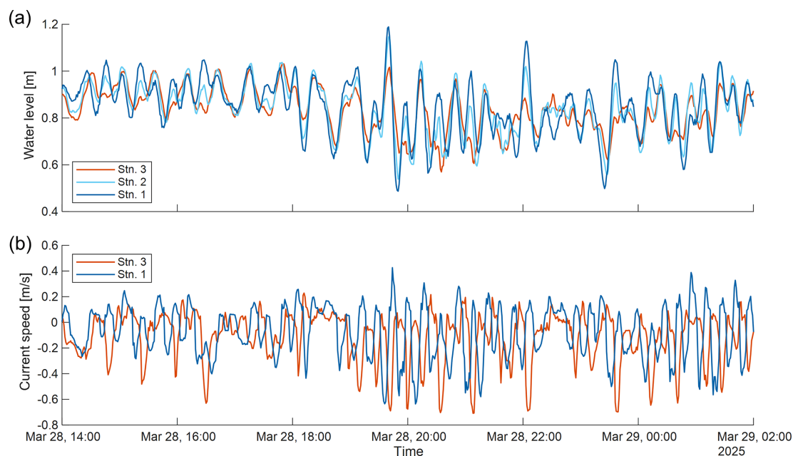
Figure 8. (a) Water level and (b) along-channel current speed during 12 h of the high-current-speed event on 28–29 March 2025. Initial data with a 1 min resolution.
