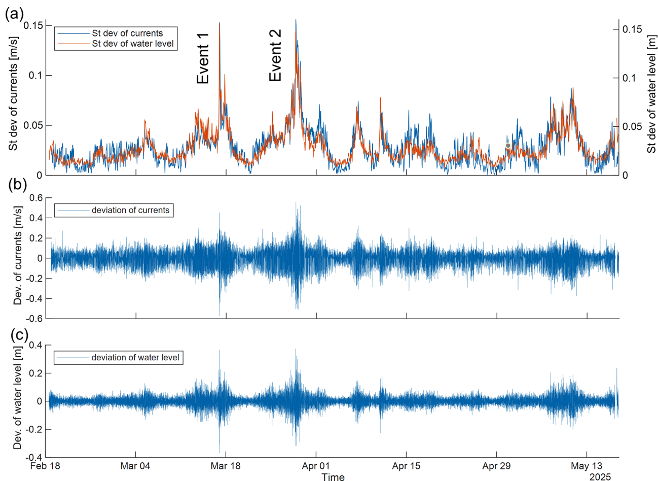
Figure 3. Joint panel of sub-hourly standard deviations of (a) current speed and water level over one-hour period, and the time series of 1 min resolution sub-hourly deviations of (b) along-channel current speed and (c) water level. Labeled are the high-speed cases Event 1 and Event 2.
