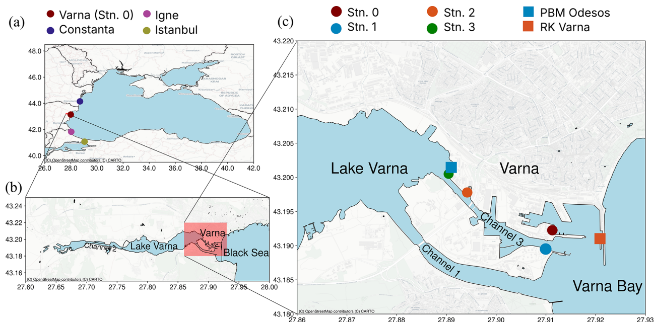
Figure 1. (a) Location of the study area, shown on the map of the Black Sea. The western coastal stations where data are shared within the Copernicus Marine Service data © European Union, 2026 are indicated on the map. (b) Map of the Varna region. (c) Map of the study area displaying the locations of the observation sites. Details of observation points are given in Table 1.
