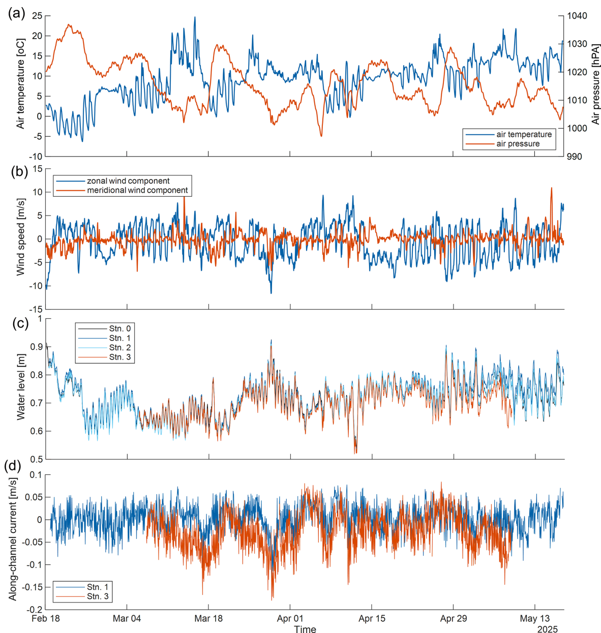
Figure 2. Time series of meteorological and oceanographic data with 1 h resolution. (a) Air temperature and air pressure, (b) zonal and meridional components of wind speed, (c) water level and (d) along-channel current speed (positive from lake to sea). Data from RK Varna (a, b) , stations from Stn. 0 to Stn. 3 (c) , and Stn. 1 and Stn. 3 (d) .
