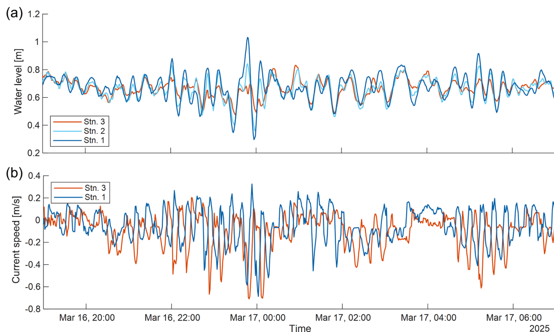
Figure 7. (a) Water level and (b) along-channel current speed during 12 h of the high-current-speed event on 16–17 March 2025. Initial data with a 1 min resolution.
