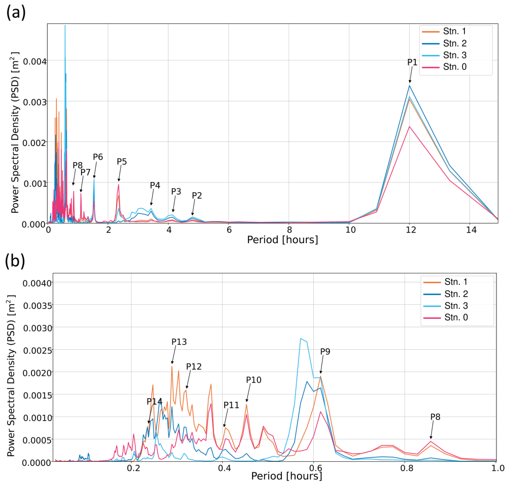
Figure 4. (a) PSD of water level at the four measurement sites of the channel in the range of periods from 2 min to 15 h using a 6 d Welch segment. (b) PSD for periods from 2 min to 1 h, computed using a 1 d Welch segment length to better resolve higher-frequency variability. Marked are the peak periods, starting from the longest period, P1, to the shortest period, P14. Main features of the oscillation peaks are given in Table 2.
