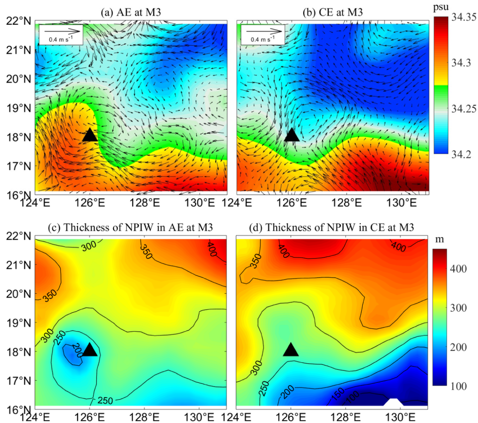
Figure 14. (a) Composite distribution of salinity (color shading) and current vectors (black arrows) averaged over the 500–700 m layer during high-salinity events generally associated with anticyclonic conditions near the M3 mooring site from CMEMS data. (b) Same as (a), but for low-salinity events generally associated with cyclonic conditions. (c) Composite thickness of the NPIW layer during high-salinity events, calculated from the 34.3 psu isohaline boundaries. (d) Same as (c), but for low-salinity events. Black triangles indicate the mooring locations.
