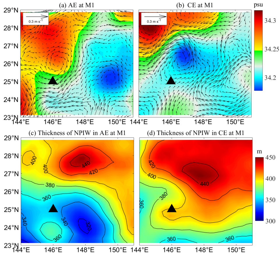
Figure 12. (a) Composite distribution of salinity (color shading) and current vectors (black arrows) averaged over the 500–800 m layer during high-salinity events generally associated with anticyclonic conditions near the M1 mooring site from CMEMS data. (b) Same as (a), but for low-salinity events generally associated with cyclonic conditions. (c) Composite thickness of the NPIW layer during high-salinity events, calculated from the 34.3 psu isohaline boundaries. (d) Same as (c), but for low-salinity events. Black triangles indicate the mooring locations.
