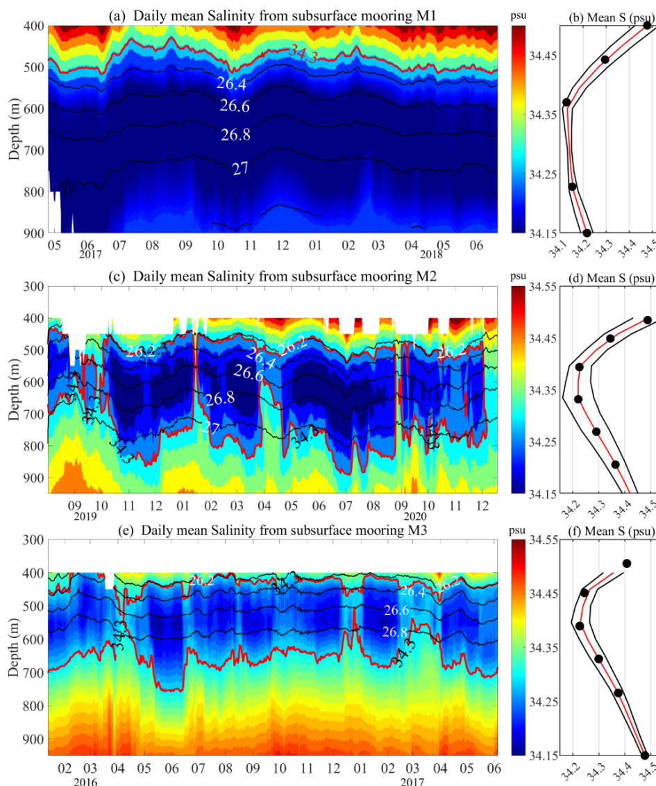
Figure 2. The observation of salinity from subsurface mooring. (a), (c) and (e) represent time series plots of salinity measured at different observation times for the three moorings, respectively. M1 is observed from April 2017–June 2018, M2 is observed from August 2019–December 2020 and M3 is observed from January 2016–June 2017. Color shading and the black lines represent the salinity and 26.2 to 27.0 \sigma_\theta isopycnal, and also red line represent the 34.3 psu in (a), (c) and (e), respectively. In (b), (d) and (f), the red line and black line represent the mean salinity and standard deviation of salinity over the observation period, respectively. The black circle in (b), (d) and (f) are represents the average depth of deployed CTDs in subsurface moorings.
