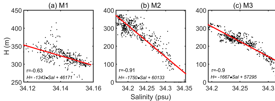
Figure 8. Scatterplots showing the relationship between NPIW layer thickness and isopycnal-averaged salinity ( 26.4\text{--}26.9\sigma_\theta ) at mooring sites M1, M2, and M3. Each point represents a daily-averaged value. Linear regression fits are shown in red line. The correlation coefficients are -0.63 , -0.91 , and -0.90 for M1, M2, and M3, respectively.
