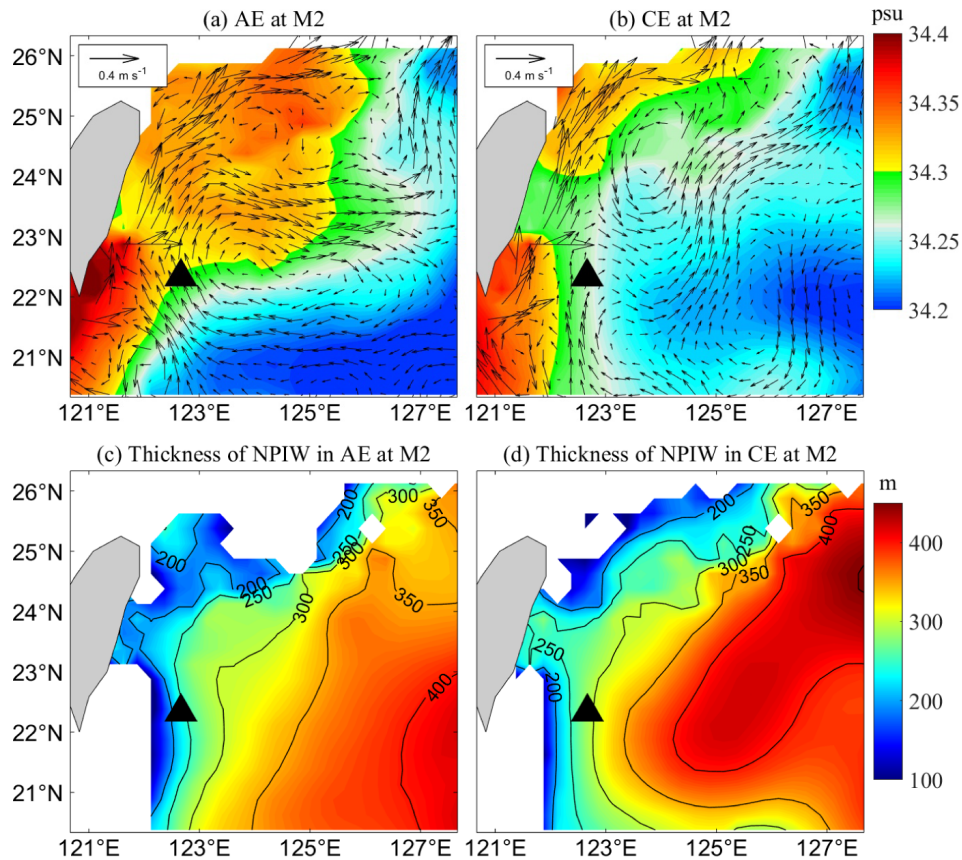
Figure 13. (a) Composite distribution of salinity (color shading) and current vectors (black arrows) averaged over the 500–800 m layer during high-salinity events generally associated with anticyclonic conditions near the M2 mooring site from CMEMS data. (b) Same as (a), but for low-salinity events generally associated with cyclonic conditions. (c) Composite thickness of the NPIW layer during high-salinity events, calculated from the 34.3 psu isohaline boundaries. (d) Same as (c), but for low-salinity events. Black triangles indicate the mooring locations.
