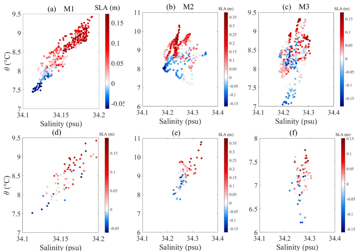
Figure 7. (a) The salinity and temperature data at M1 are displayed in a T – S scatter diagram with colors denoting the associated sea level anomalies (SLAs). (b) and (c) are same as (a), but for M2 and M3. (d), (e) and (f) are T – S plots of 500–800 m averaged temperature and salinity data from CMEMS product in the intermediate layer corresponding to the locations of M1, M2, and M3, respectively.
