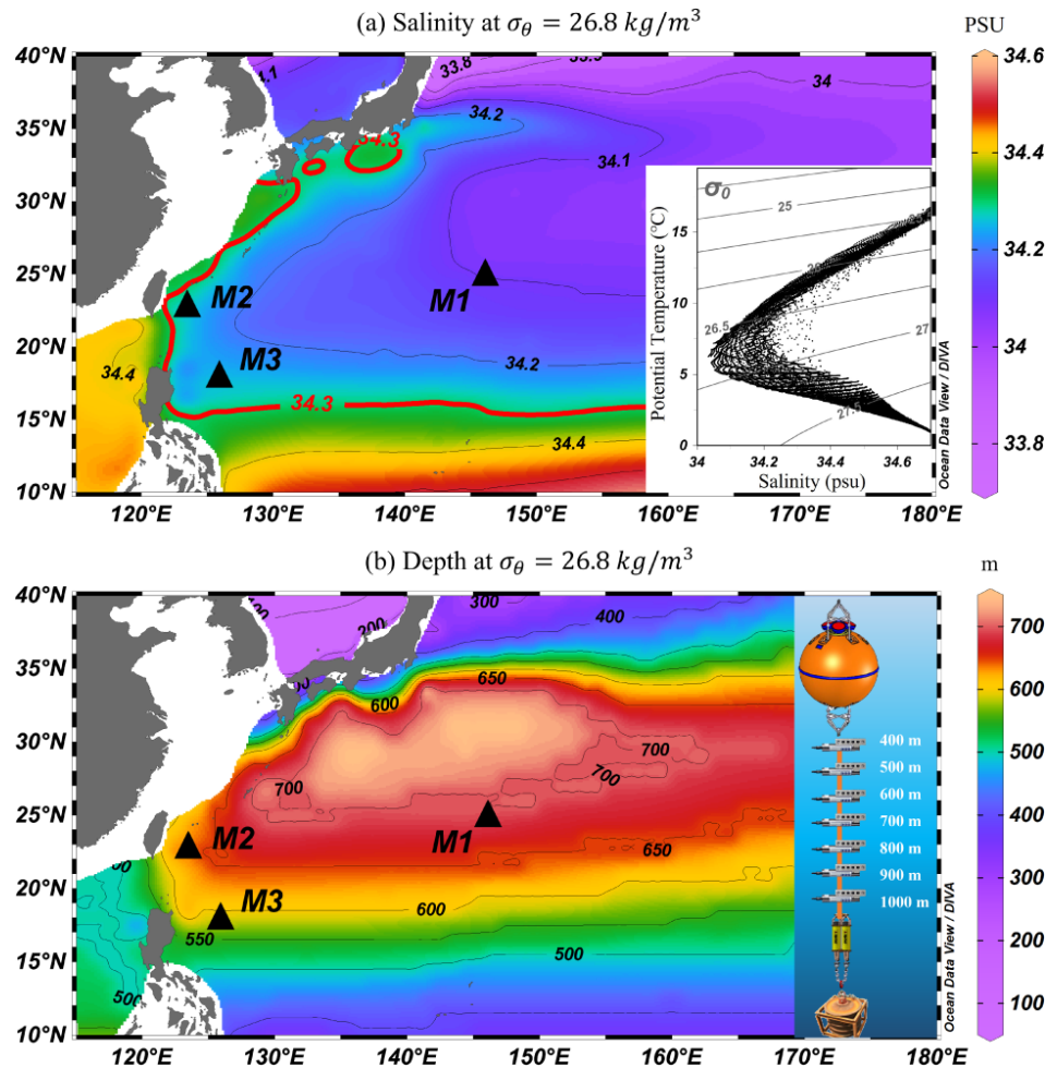
Figure 1. Distribution of salinity (a) and depth (b) along the 26.8\sigma_\theta isopycnals at Northwestern Pacific. The T - S scatter plot in the lower-right corner of (a) illustrates the vertical distribution of NPIW. The color shading and black line in (a) and (b) represent the salinity and depth, respectively. The right-hand side of (b) shows a schematic diagram of the CTD deployment with mooring. The red contours of 34.3 psu is represent the NPIW range from Talley (1993) and You (2003). The black triangle is the mooring location: Mooring 1 (M1), Mooring 2 (M2) and Mooring 3 (M3). Salinity and depth in the Fig. 1 are taken from climatological averaged data from World Ocean Atlas 2023 (WOA23), NOAA National Centers for Environmental Information, and plot with Ocean Data View (Schlitzer, Reiner, Ocean Data View, https://odv.awi.de , last access: 28 July 2026, 2022).
