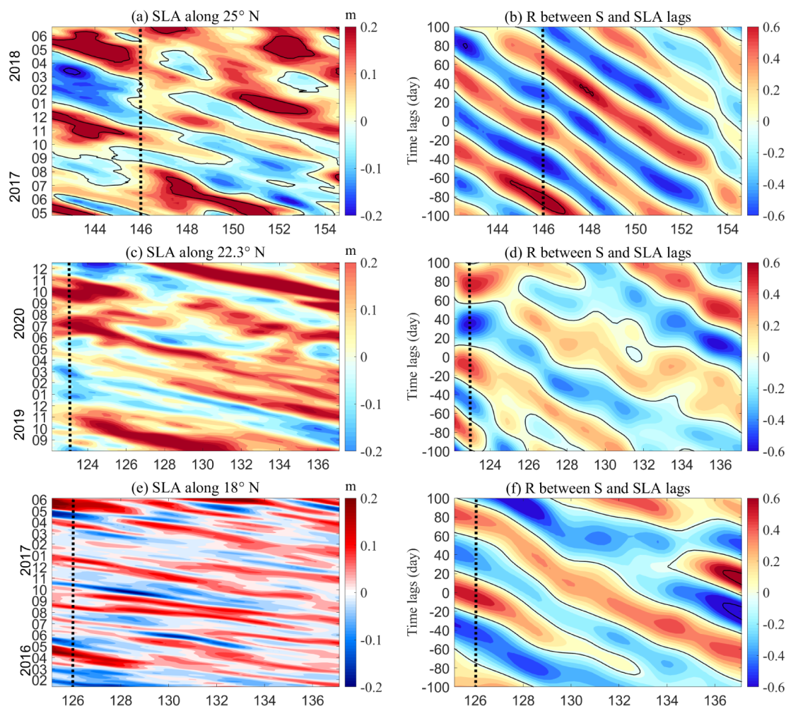
Figure 9. (a) Temporal evolution of sea level anomalies (SLAs) across longitudes at 25° N, as illustrated by the contour plots; (b) The correlation coefficient between salinity at M1 and SLA at different time lags, the vertical coordinates -100 to 100 d in (b) represent SLA lagging salinity for 100 d and SLA exceeding salinity for 100 d, respectively. (c) and (e) are same as (a), but its along 22.3° N and 18° N, respectively. (d) and (f) are same as (b), but for salinity from M2 and M3, respectively. Black contours in Fig. 9b, d, and f represent the zero isolines. The black dash line represent the location of M1, M2 and M3, respectively. The SLA data shown in this figure were obtained from the CMEMS dataset introduced in the Methods section.
