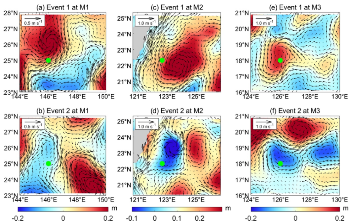
Figure 10. (a) and (b) are selected SLAs and surface geostrophic current maps corresponding to the moments of Event 1 and Event 2 observed from M1, respectively, where time of Event 1 corresponds to 15 October 2017 in Fig. 6a, and Event 2 corresponds to 29 November 2017 in Fig. 6a. (c) and (d) are same as (a) and (b), but for mooring site M2, where time of Event 1 and Event 2 at M2 corresponding to 20 April and 5 March 2020 showed in Fig. 6b. (e) and (f) are same as (a) and (b), but for mooring site M3, where time of Event 1 and Event 2 at M3 corresponding to 10 April 2016 and 15 April 2017 showed in Fig. 6c. The green dots denotes the mooring site, the colors shading represent the SLAs and the arrows indicate the surface geostrophic current.
