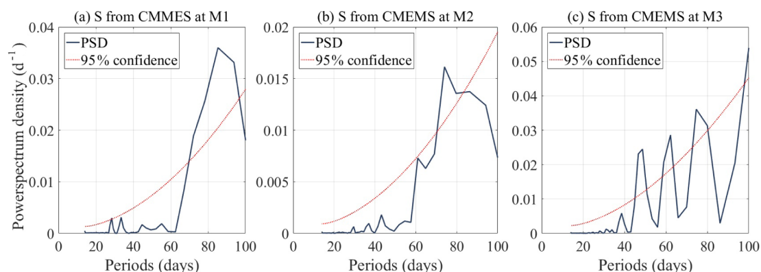
Figure 11. (a) The power spectrum density of 500–800 m averaged salinity at location of M1 from CMEMS data. (b) and (c) are same as (a), but for location of M2 and M3, respectively. The red dash line represent the 95 % confidence level.
