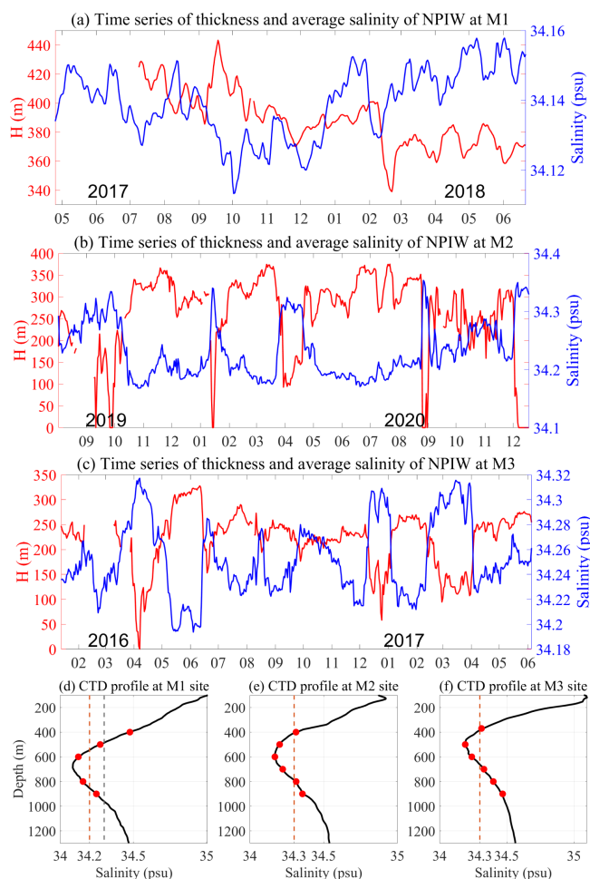
Figure 4. Time series of thickness and averaged salinity of NPIW at M1 (a), M2 (b) and M3 (c). The layer thickness was estimated as the vertical distance between the upper and lower selected isohalines. The 34.2 psu isohaline was used at M1, whereas the 34.3 psu isohaline was used at M2 and M3. The average salinity between the 26.4 and 26.9 \sigma_\theta isopycnal was used to represent the salinity characteristics of the NPIW. (d–f) Shipboard CTD salinity profiles near M1, M2, and M3, respectively. The black curves denote the full-resolution shipboard CTD salinity profiles, and the red circles indicate salinity values sampled from these profiles at the nominal depths of the moored CTD sensors. The orange dashed lines mark the selected isohaline used for estimating the thickness of the low-salinity intermediate layer: 34.2 psu at M1 and 34.3 psu at M2 and M3. The grey dashed line in panel (d) marks 34.3 psu for comparison. These profiles show a well-defined low-salinity intermediate layer and relatively smooth salinity variations across the selected isohaline intervals, supporting the use of local linear interpolation between adjacent moored CTD sensors.
