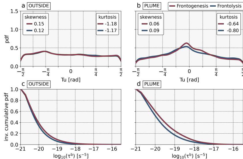
Figure 8. Statistics of modeled Tu and \tau^b . (a, b) Pdf of Tu separated between gradients showing frontogenesis (red) and frontolysis (blue), for (a) OUTSIDE and (b) the PLUME. (c, d) Inverse cumulative pdf of frontogenesis (red) and frontolysis (blue), for (c) OUTSIDE and (d) the PLUME.
