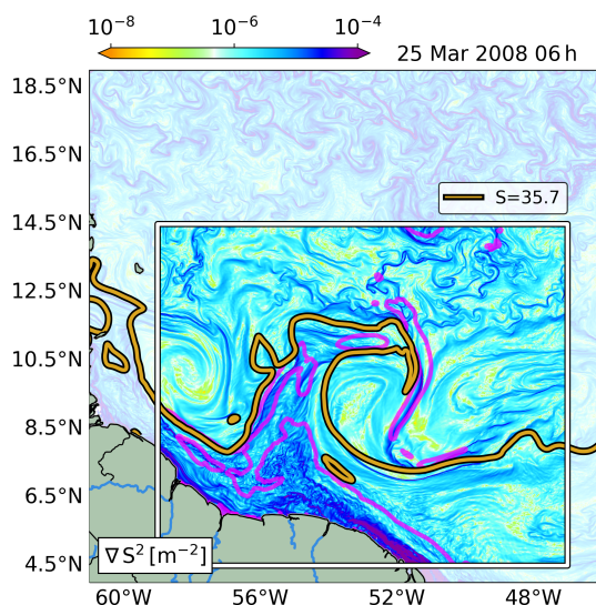
Figure C1. Model surface salinity gradient on 25 March 2008, 6 h. The plume region is delimited by the isohaline representing the 0.25 quantile of the salinity probability distribution (golden line). Purple lines represent the 20 % strongest mesoscale SSS gradient.
