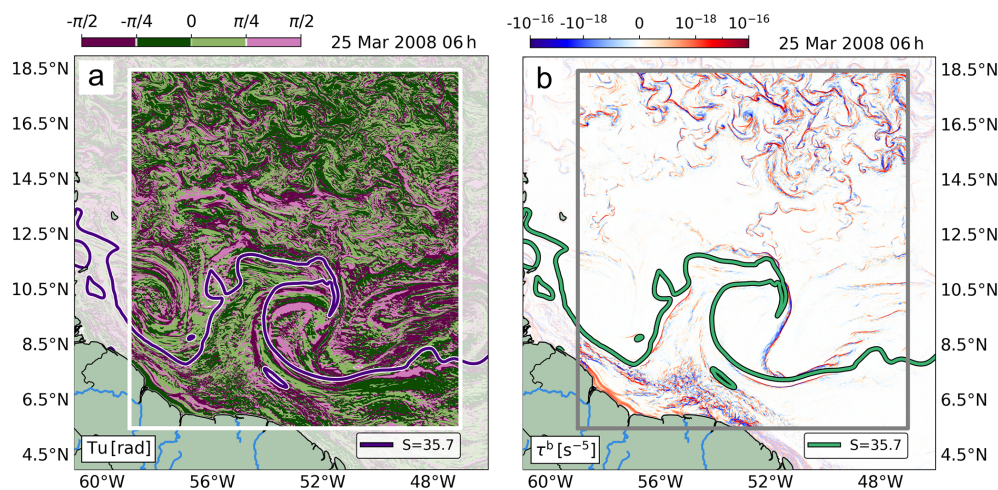
Figure 9. Spatial distribution of (a) the Turner Angle Tu and (b) the Frontogenetic Tendency of Buoyancy \tau^b for the snapshot on 25 March 2008, 6 h. The PLUME region is delimited by the isohaline representing the 0.25 quantile of the salinity probability distribution (dark blue and green lines).
