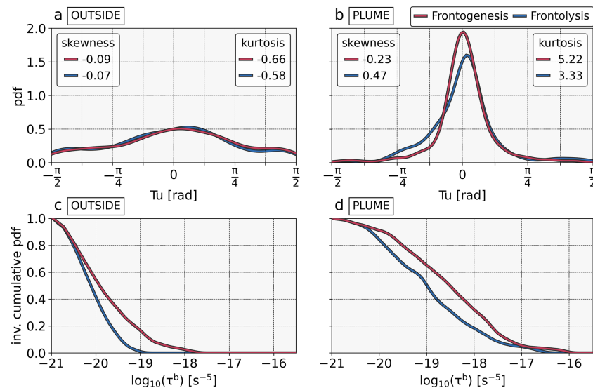
Figure 4. Statistics of observed Tu and \tau^b at \ell = 1 km. (a, b) Pdf of Tu separated between gradients showing frontogenesis (red) and frontolysis (blue), for (a) OUTSIDE and (b) the PLUME. (c, d) Inverse cumulative pdf of frontogenesis (red) and frontolysis (blue) for (c) OUTSIDE and (d) the PLUME.
