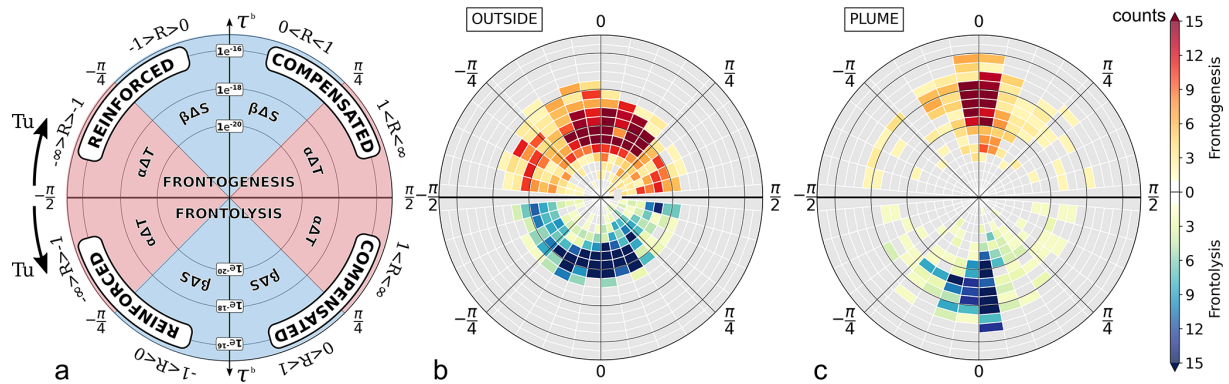
Figure 3. Overview of observed gradients. (a) Schematic diagram mirroring gradients related to frontogenesis (top) and frontolysis (bottom). Radial distances represent the strength of \tau^b [ \text{s}^{-5} ]. Azimuthal distances represent Turner angle Tu (clockwise from -\frac{\pi}{2} for frontogenesis and counterclockwise for frontolysis), where quadrants indicate if density gradients are driven by salinity (blue) or temperature (red) and if they compensate or reinforce each other. (b, c) Saildrone surface density variations at \ell = 1.0 km scale OUTSIDE (b) ; 1964 samples) and inside the PLUME (c) ; 810 samples). Colors indicate the number of gradients sampled for each azimuthal and radial bin.
