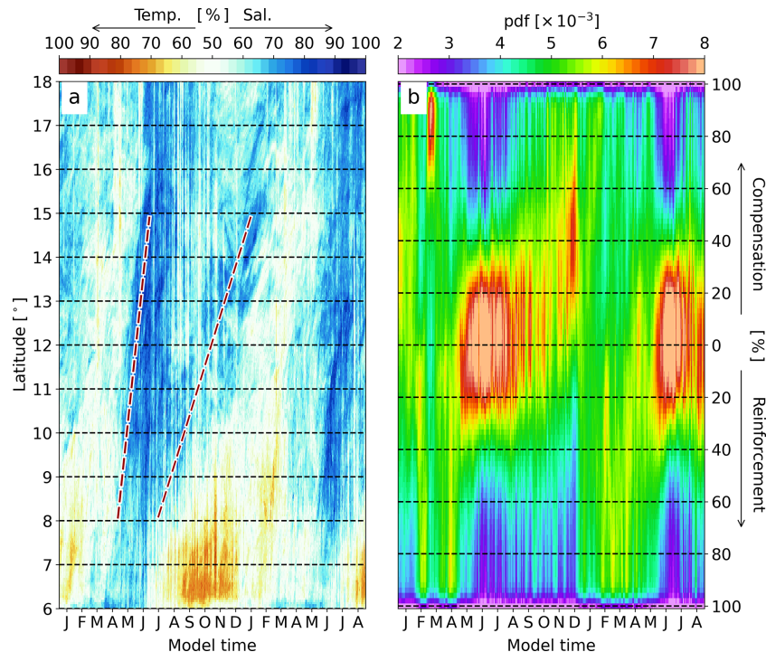
Figure 10. (a) Hovmöller diagram of the percentage of salinity (% Sal.) vs. temperature (% Temp.) dominance in the density ratio during the plume propagation northward (59–47° W; 6–18° N). Model time starts on 1 January 2008. (b) Daily timeseries of the probability density function of the percentage of compensation or reinforcement in the density ratio within the PLUME region.
