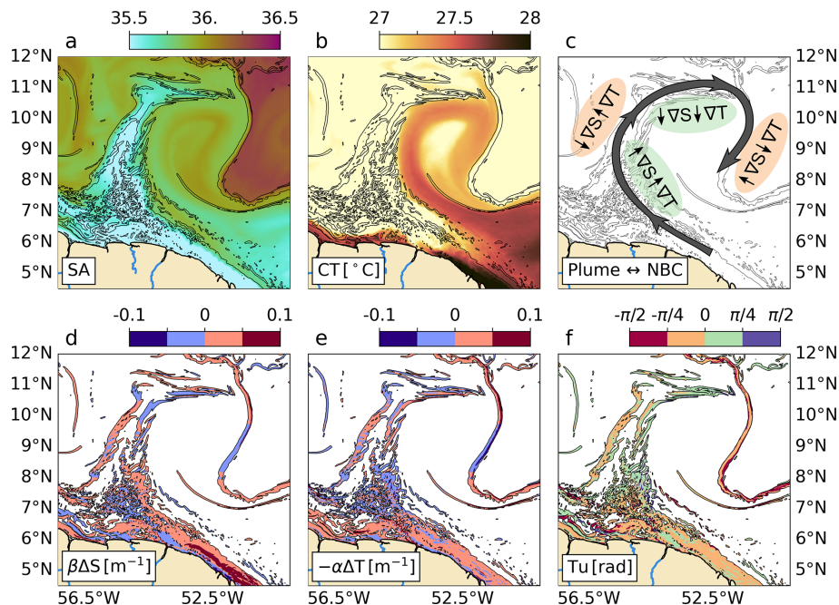
Figure 11. Interaction of the NBC and the Amazon Plume zoomed in from the model on 25 March 2008, 6 h. (a) SA: Absolute salinity; (b) CT: Conservative Temperature; (c) Schematic of compensation (green) and reinforcement (orange) developing on opposite sides of the low-salinity filament; (d) contribution of salinity to density variation; (e) contribution of temperature to density variation; (f) Tu: Turner angle. The blowout of T – S gradients in (d–f) selects areas where |\beta\Delta S| \geq 0.01 \text{ m}^{-1} , where thin black contours represent \beta\Delta S = 0.01 \text{ m}^{-1} . In (d–f) , colors delimit regions of \beta\Delta S \geq 0.01 \text{ m}^{-1} .
