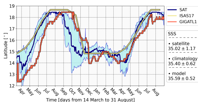
Figure B1. Northernmost position of the 36 isohaline between 14 March and 31 August from satellite (dark blue line mean with 80 % of the distribution in light blue), climatology (light yellow line), and model (red line). For the satellite data, five 18-month series (light grey lines) span data from 2016 to 2021. The monthly climatology is reorganized to display 18 months of data. The model years (March 2008–August 2009) are referenced due to the data used for forcing. Product keys: SAT – satellite product is a regional product distributed by CATDS CEC (Boutin et al., 2022), providing a combination of SMOS and SMAP sea surface salinity data; ISAS17 – stable (delayed time) Argo climatology distributed by Argo France (Kolodziejczyk et al., 2023); GIGATL1 – CROCO numerical simulation (Gula et al., 2021).
