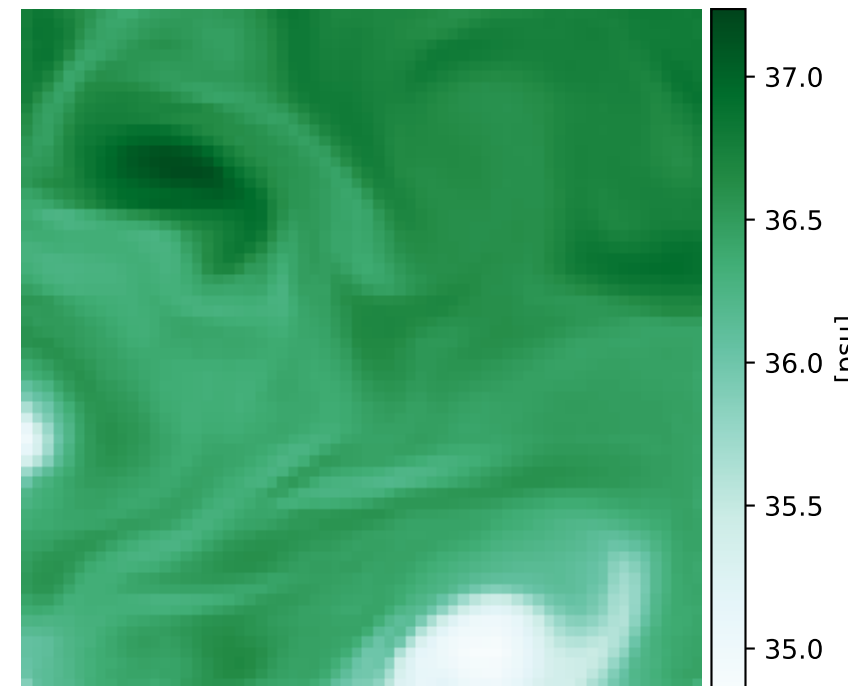
Sample 6 (1/12°)
