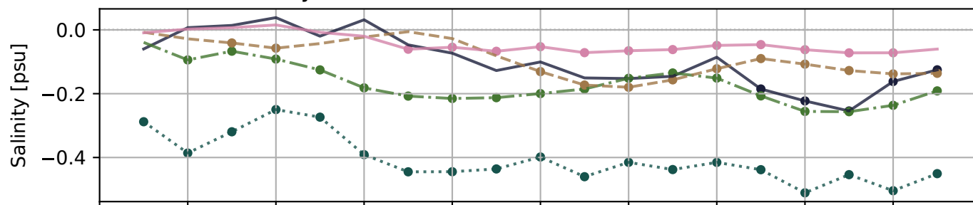
(a) Surface salinity
