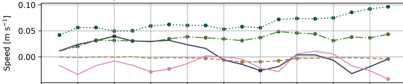
(c) Horizontal speed modulus
