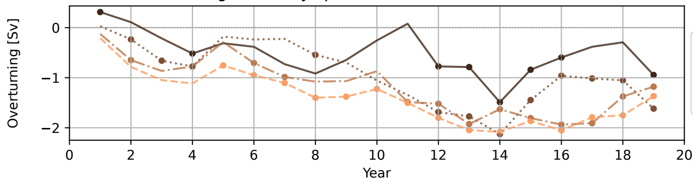
(e) Max overturning in density-space
