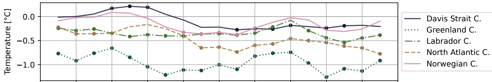
(b) Surface temperature
