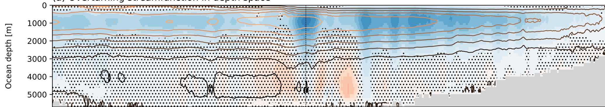
(a) Overturning streamfunction in depth space
