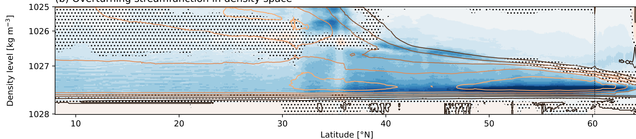
(b) Overturning streamfunction in density space
