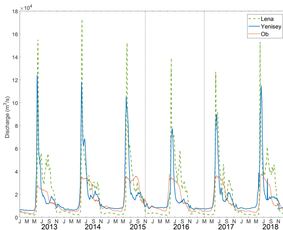
Figure 8. Time series of river discharge from the Lena (green), Yenisey (blue), and Ob (orange) Rivers from 2013 to 2018. Dashed black lines indicate the period of the freshening event in the Eurasian Basin. Note the increased freshwater discharge from the Lena and Yenisey Rivers before the event. Data source: The Arctic Great Rivers Observatory: https://arcticgreatrivers.org/ , last access: 15 September 2025.
