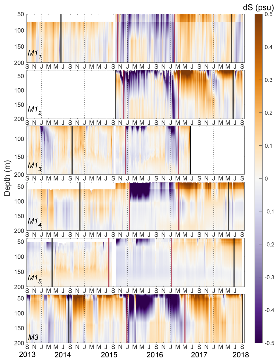
Figure 2. Depth–time distributions of anomalous salinity (relative to the 2013–2018 mean) from six mooring locations in the eastern Eurasian Basin (see positions in Fig. 1) from 2013 to 2018. Vertical dotted lines mark 1 January as the start of each year. Vertical red lines indicate the freshening event (2015–2017), and solid black lines mark the periods before and after the event, used for comparative analysis. White gaps indicate missing data.
