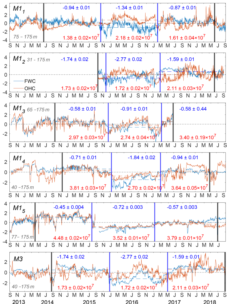
Figure 6. Normalized time series of freshwater content (FWC, m; blue) and ocean heat content (OHC, \text{J m}^{-2} ; orange) averaged over the depth range (indicated in the bottom left of each panel) for six mooring locations in the eastern Eurasian Basin. FWC values are multiplied by -1 so that freshening appears as a negative anomaly, aligning visually with changes in OHC. Horizontal dashed lines represent the mean values for each period. Mean \pm 3 standard errors are shown in dark blue for FWC and in red for OHC. Vertical dark blue lines indicate the period of the freshening event; the vertical black lines mark the periods before and after the event.
