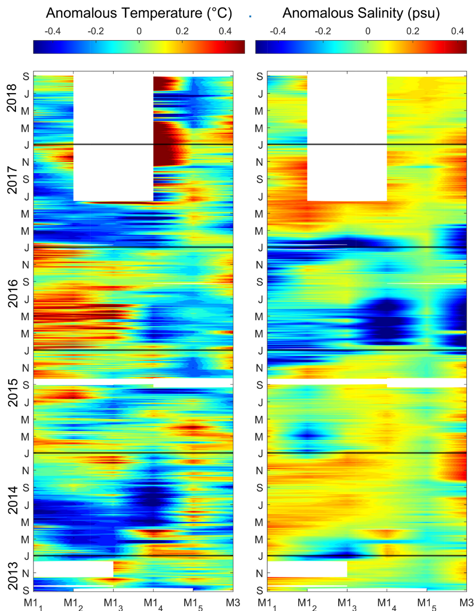
Figure 3. Hovmöller diagrams of temperature and salinity anomalies (relative to the 2013–2018 mean) at 77 m depth for six mooring locations in the eastern Eurasian Basin. The 77 m depth was selected based on the shallowest continuous salinity record across all moorings. The horizontal axis represents mooring site labels, and the vertical axis shows time (September 2013 to September 2018). Horizontal black lines mark the start of each year. White gaps indicate missing data.
