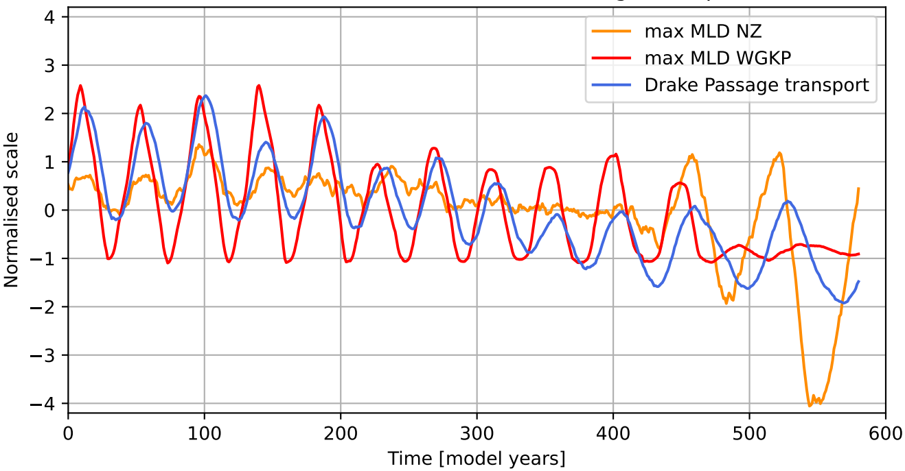
MLD NZ, MLD WGKP and Drake Passage transport
