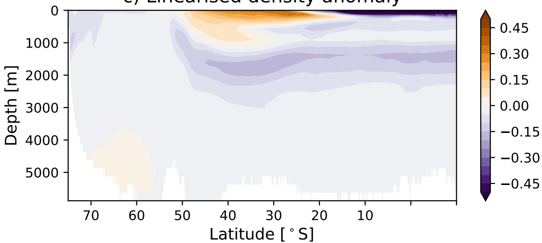
c) Linearised density anomaly
