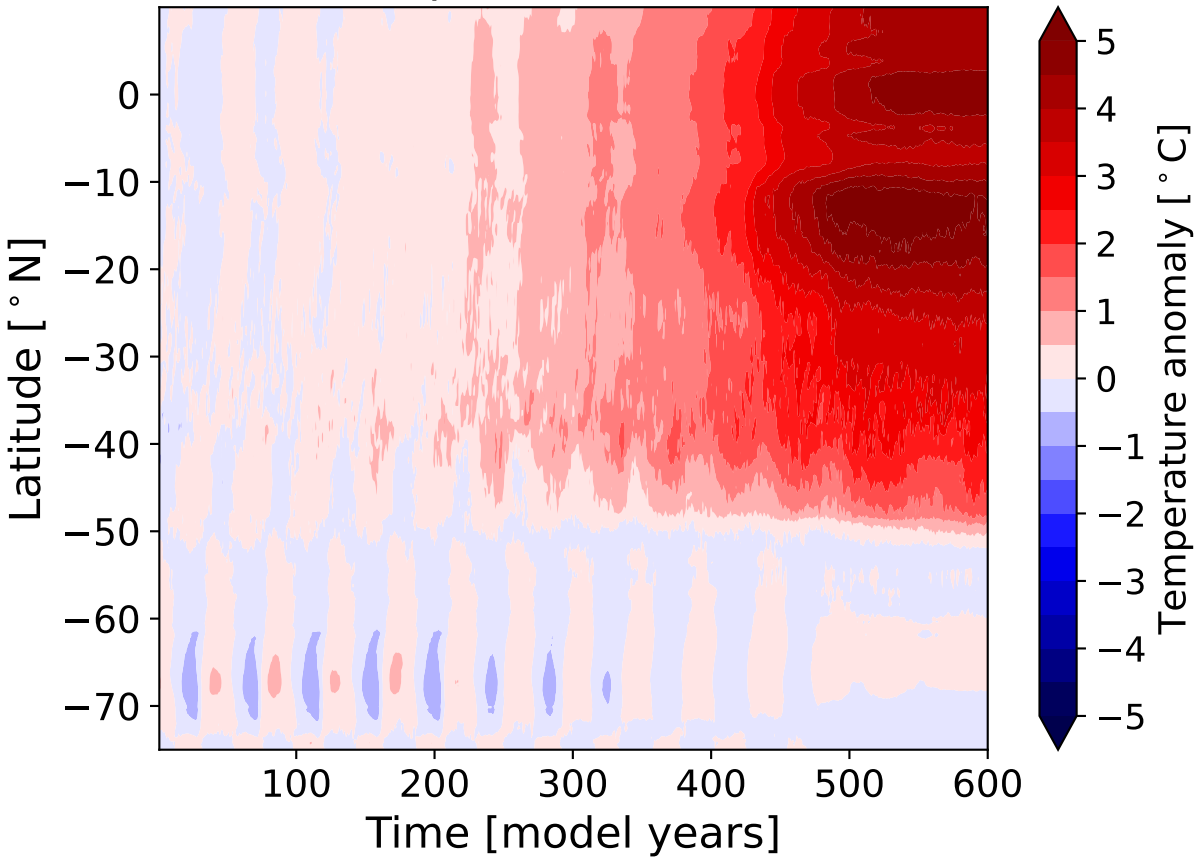
a) Temperature anomalies
