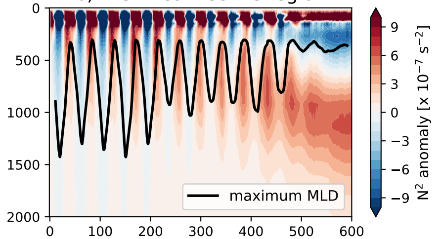
d) PA convective region
