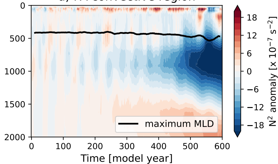
d) PA convective region
