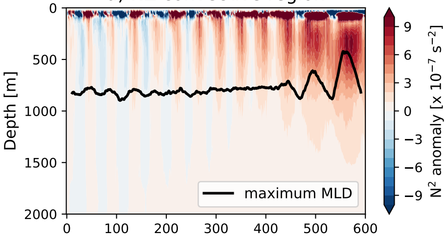
c) AU convective region
