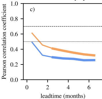
Number of MHW days per month
