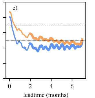
Fraction of SWP2 in MHW state
