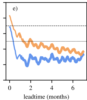
Fraction of NC_EEZ in MHW state
