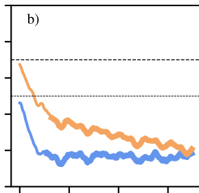
Severity monthly max
