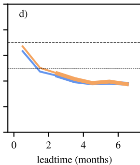
Severity monthly max
