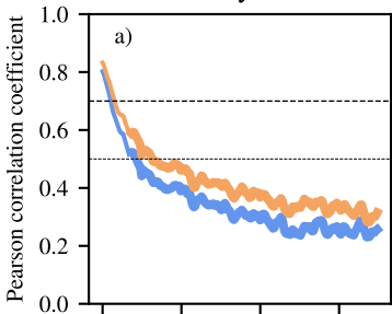
Number of MHW days per month
