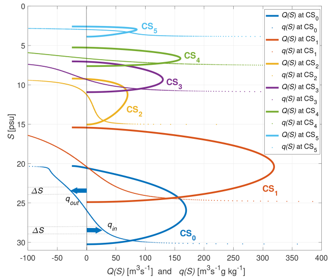
Figure 2. Volume transports Q(S) (solid curves) and exchange profiles (dotted curves) q(S) sorted by salinity classes are computed at cross-sections CS_i . Note the inversion of the vertical axis.
