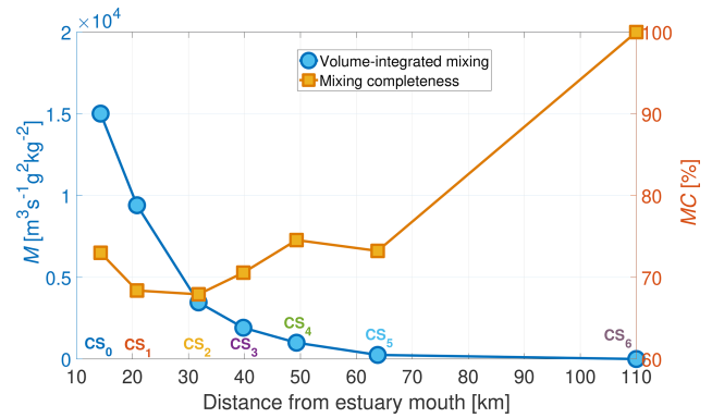
Figure 5. Volume-integrated mixing (left y-axis; dark blue curve, circles) and mixing completeness (right y-axis; dark yellow curve, squares).
