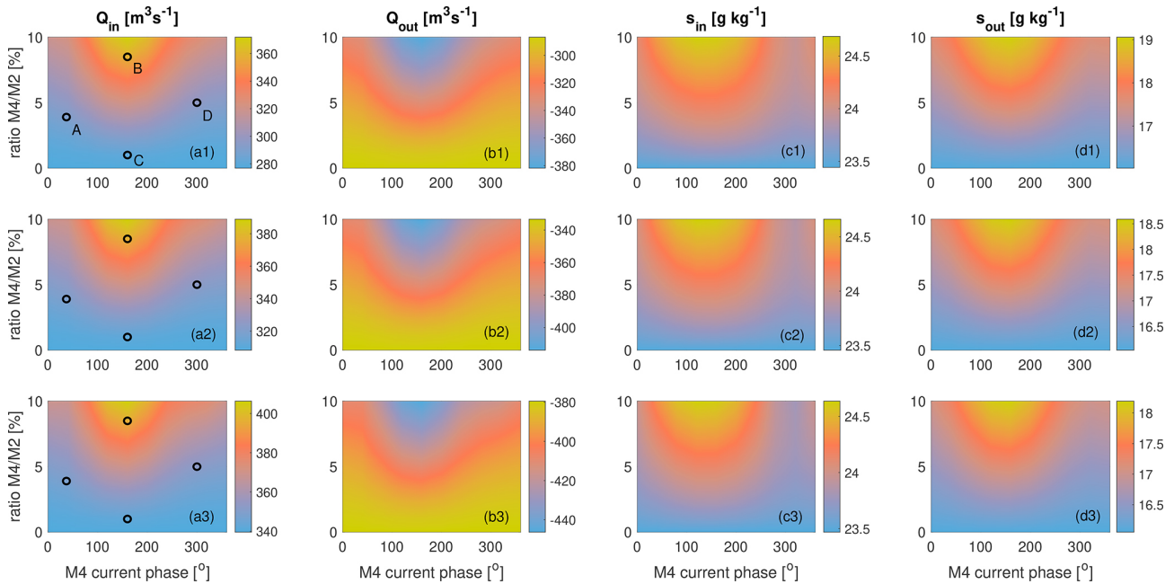
Figure 7. Sensitivity of incoming (panels a1 , a2 , and a3 ) and outgoing volume transports (panels b1 , b2 , and b3 ) and salinities for inflows (panels c1 , c2 , and c3 ) and outflows (panels d1 , d2 , and d3 ) to ratio between M4 and M2 current amplitudes ( u_b/u_a ) and to M4 current phase ( \varphi_b ). First, second and third row of panels correspond with R = 10 \text{ m}^3 \text{ s}^{-1} , R = 25 \text{ m}^3 \text{ s}^{-1} , and R = 40 \text{ m}^3 \text{ s}^{-1} , respectively. Black circles and capital letters indicate example cases in the parameter space shown in Fig. 8.
