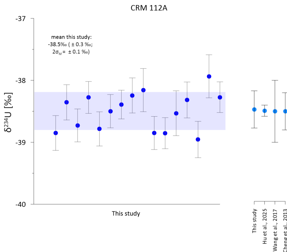
Figure 2. The CRM112A standard was repeatedly measured. The mean value of -38.5\text{‰} \pm 0.3\text{‰} is in line with other studies (Cheng et al., 2013; Wang et al., 2017; Hu et al., 2025).
