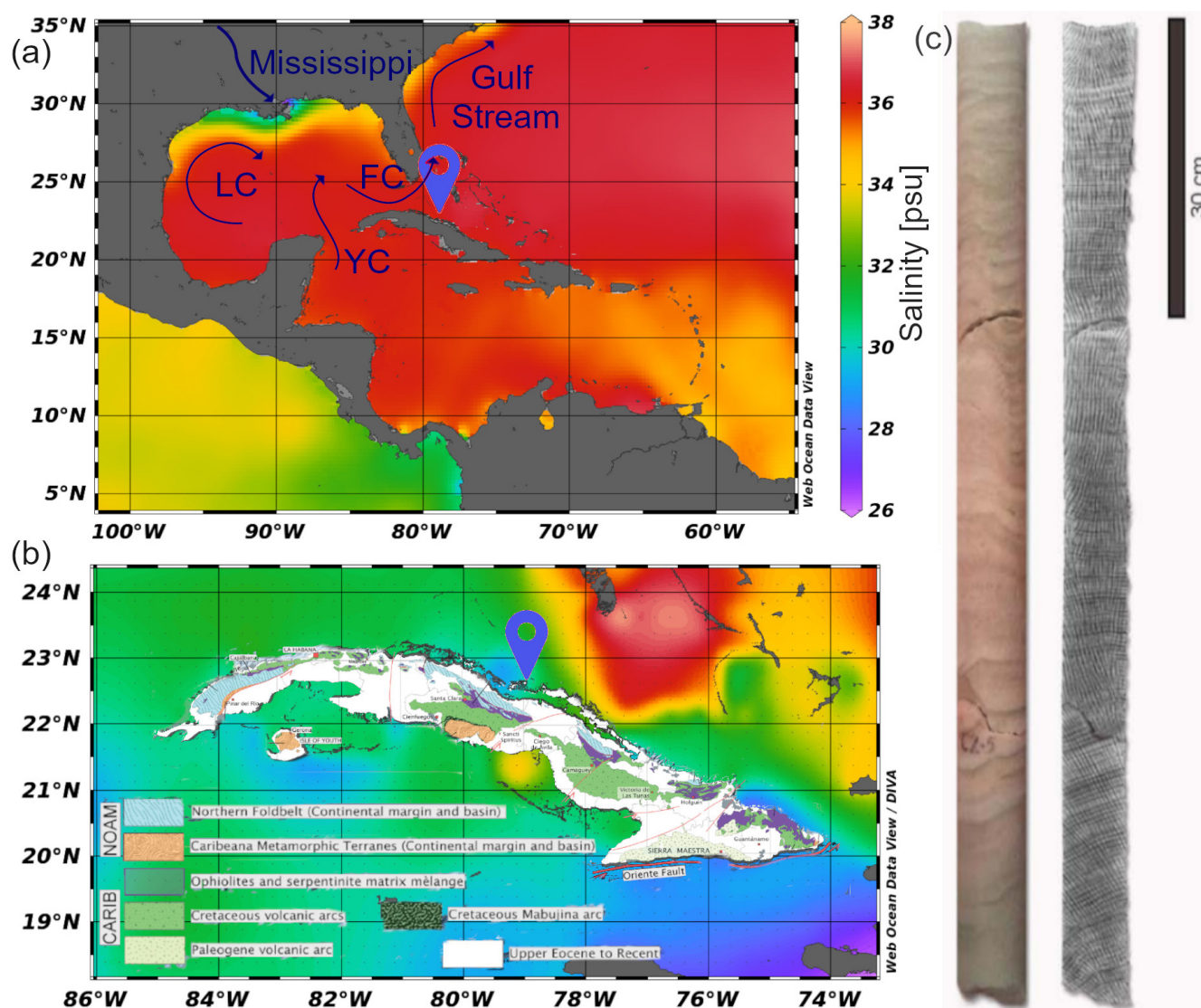
Figure 1. (a) Caribbean annual sea surface salinity (Schlitzer, 2025) with the location of the selected coral core on the northern shore of Cuba, directly influenced by the Florida Current (FC) travelling eastwards from Yucatan Current (YC) and the Gulf of Mexico forming the Gulf Stream. The Loop Current (LC) carries the less saline Mississippi water towards the coral. (b) Annual sea surface salinity off the coast of Cuba (Schlitzer, 2025); less salinity is observed at the core location due to terrestrial runoff. With generalized geologic-tectonic map of Cuba modified from Iturralde-Vinent et al. (2016). (c) X-ray image of the slab used in the optical densitometry analysis and photograph of the analysed core (CSM-1) with visible green banding.
