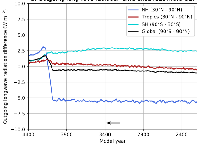
b) Outgoing longwave radiation difference (backward QE)
