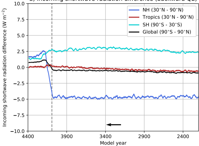
a) Incoming shortwave radiation difference (backward QE)
