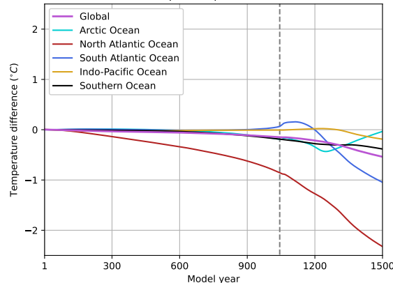
f) Upper 1000 m temperature, LR-POP
