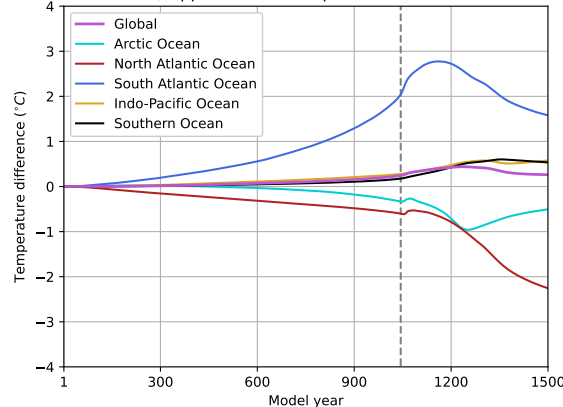
i) Below 1000 m temperature, LR-POP
