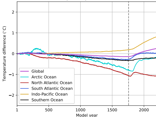
d) Upper 1000 m temperature, LR-CESM
