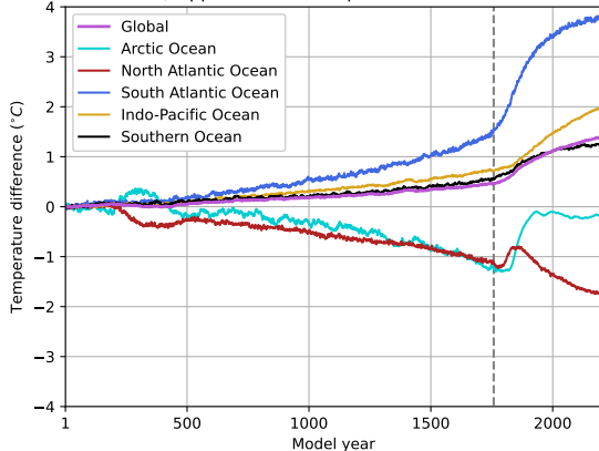
g) Below 1000 m temperature, LR-CESM
