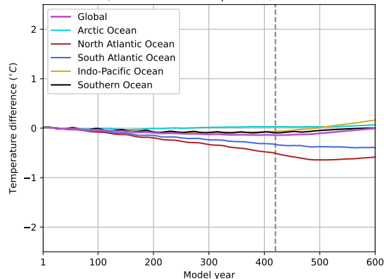
h) Below 1000 m temperature, HR-POP
