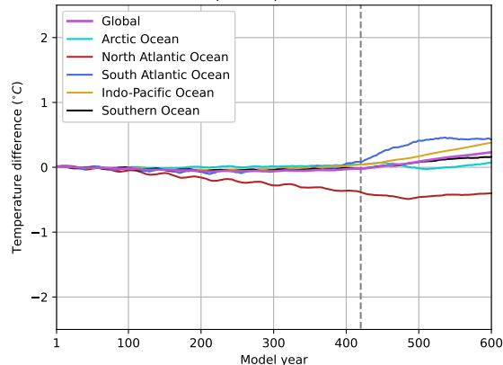
e) Upper 1000 m temperature, HR-POP
