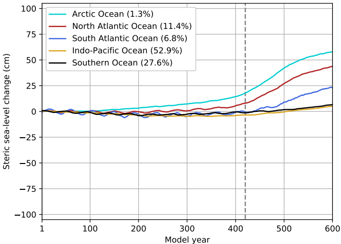
c) Steric sea level, HR-POP
