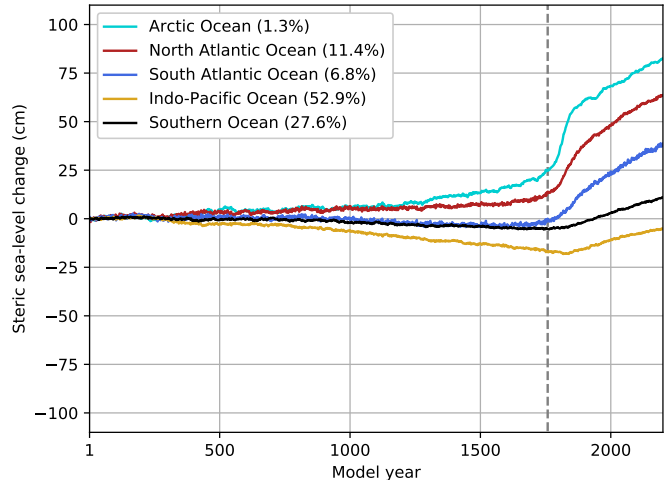
d) Steric sea level, LR-POP
