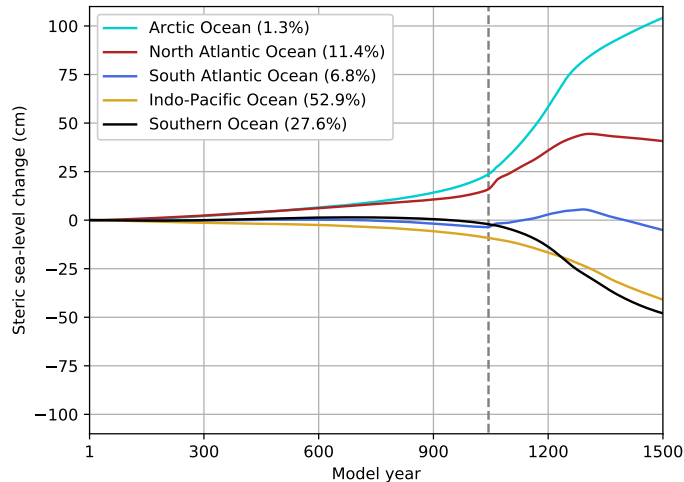
d) Steric sea level, LR-POP
