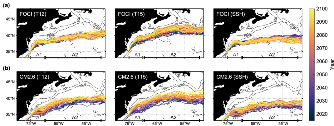
Figure 4. Annual mean location of the GS path based on temperature (T12 and T15) and SSH criteria in the warming simulations of FOCI (a) and CM2.6 (b). Colors indicate different years from 2015 to 2100. Regions A1 and A2 (shown along the x axis) indicate the longitude bands over which latitudes are averaged in Fig. 5.
