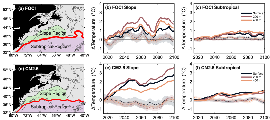
Figure 6. Changes in seawater temperature in the slope and subtropical regions of the northwest North Atlantic from the FOCI and CM2.6 models. The left panels (a, d) show the defined regions: the slope region (green) and the subtropical region (purple) with the red contour marking the mean Gulf Stream path from the control simulation. The middle (b, e) and right (c, f) panels depict the temperature change ( \Delta Temperature) relative to the 2015 annual mean. Solid lines correspond to the warming runs, and dotted lines to the control runs, with shaded areas showing one standard deviation around the annual mean (natural variability). The top row (a–c) shows results from FOCI, and the bottom row (d–f) shows results from CM2.6. Trend statistics are provided in Table S2.
