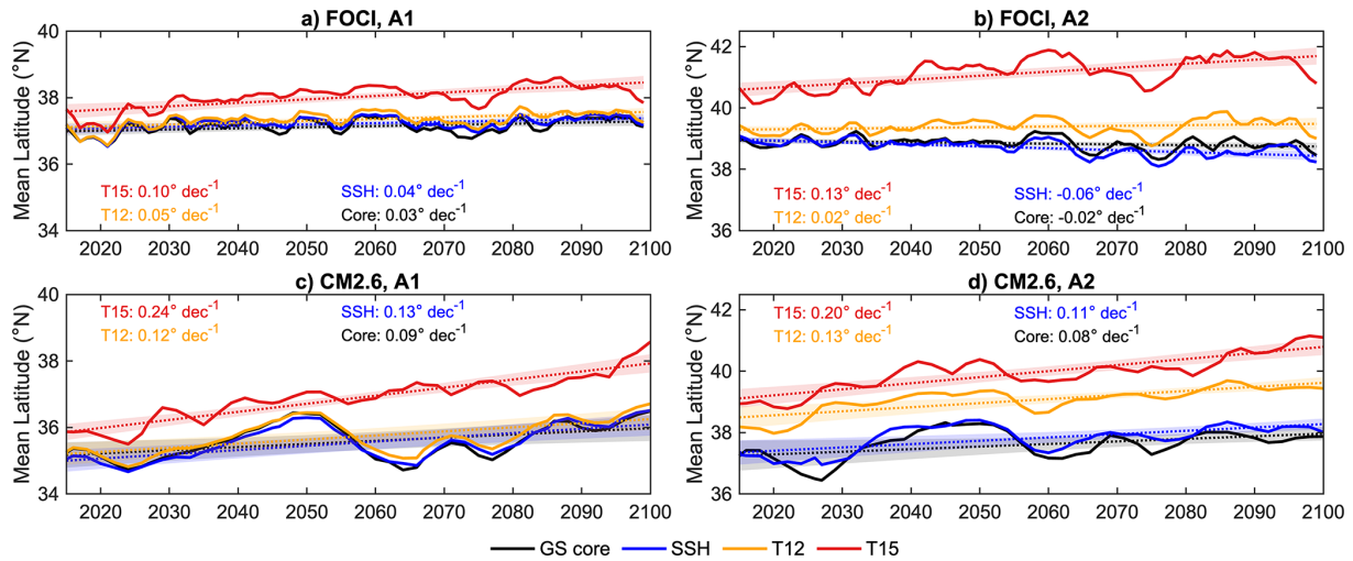
Figure 5. Mean latitude of the temperature-based (T12 and T15) and SSH-based Gulf Stream path criteria averaged over two regions: A1 (75 to 70° W, grey bracket in Fig. 4) and A2 (71 to 50° W, black bracket in Fig. 4) in FOCI (a, b) and CM2.6 (c, d) simulations. Solid lines show the annual mean latitude of each proxy, along with the reference Gulf Stream core position (GS core). Dotted lines indicate the corresponding linear trends, and shaded bands represent the 95 % confidence interval of the fitted mean trend. Trend magnitudes (in ° latitude per decade) are reported within each panel for each proxy. Trend statistics are provided in Table S1.
