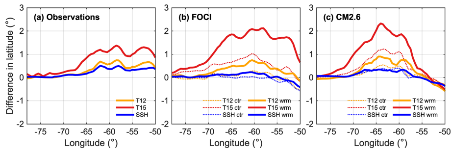
Figure 3. Differences between the GS position estimated by different criteria and the latitude of maximum velocity across different longitudes under control (ctr; dotted lines) and warming scenarios (wrm; solid lines) for observational data (a) and the FOCI (b) and CM2.6 (c) climate models in 2015. The orange (T12) and red (T15) lines correspond to the two temperature-based criteria, and the blue (SSH) lines indicate the SSH-based criterion.
