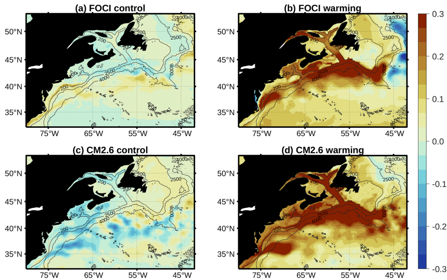
Figure 1. Linear trends in annual-mean bottom (or 200 m where the water column is deeper than 200 m) temperature between 2015 and 2100 for (a) FOCI control, (b) FOCI warming, (c) CM2.6 control, and (d) CM2.6 warming simulations. Trends are calculated from annual means.
