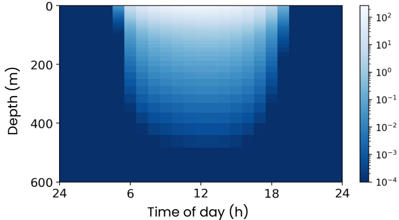
(a) Irradiance ( \text{W m}^{-2} )
