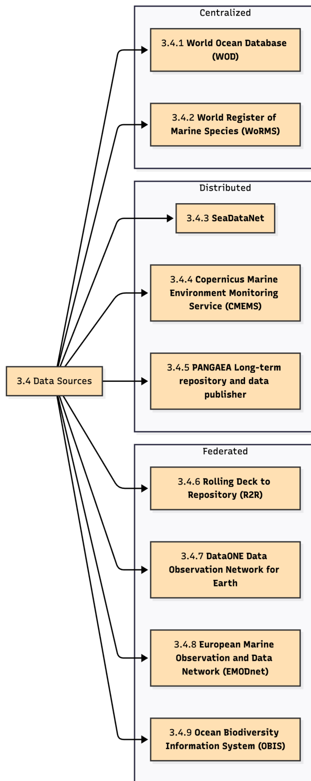
Figure 4. A diagram summarizing the examples for ocean data sources discussed in Sect. 3.4. The exemplified data sources are organized according to their infrastructural approach (namely federated, distributed and centralized).
