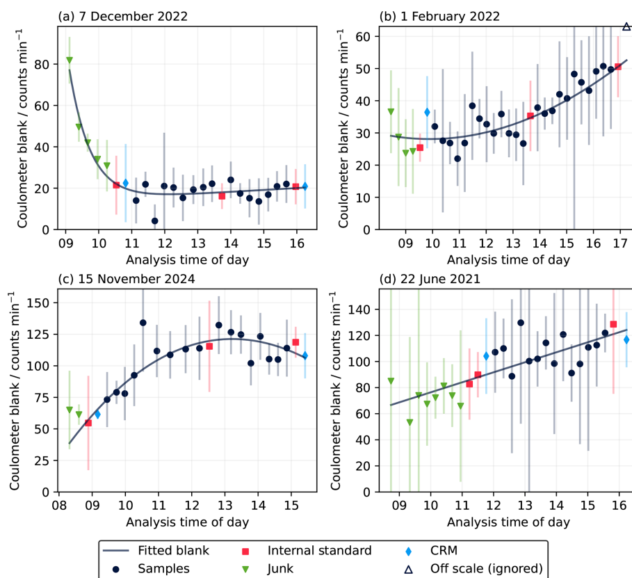
Figure 2. Equation (2) fitted to per-measurement blanks for four different analysis sessions in our test dataset (red squares; Sect. 2.6). Error bars show the standard deviation in the blank at each point, \sigma(b_m) . (a) Shows the ideal behaviour of high initial blank which declines to a stable, roughly constant value after a few hours. (b) and (c) show concave and convex patterns that are sometimes observed but can still be fitted by Eq. (2); (b) includes an off-scale point that was excluded for fitting. (d) shows an example where ignoring the exponential term in Eq. (2) gives a better fit (i.e., linear). Equivalent plots for all analysis sessions in the test datasets are available in the Supplement.
