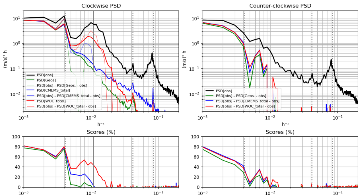
Figure 5. Same as Fig. 4, averaged between 5 and 10° N with vertical solid line indicating the inertial frequency at 7.5° N.
