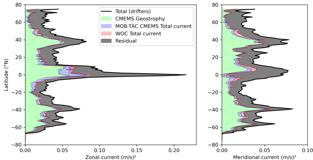
Figure 6. Black lines: variance of the observed surface current (zonal component on the left, meridional on the right) as a function of latitude averaged globally for the drifter database between 2017 and 2020. The green, blue and red lines represent the explained variance of the CMEMS geostrophy, the CMEMS MOB-TAC total current and the WOC total current. The explained variance is defined as the total variance (black) minus the variance reduction after applying the different current estimates. The filled colors indicate the relative amount of additional explained variance between successive products.
