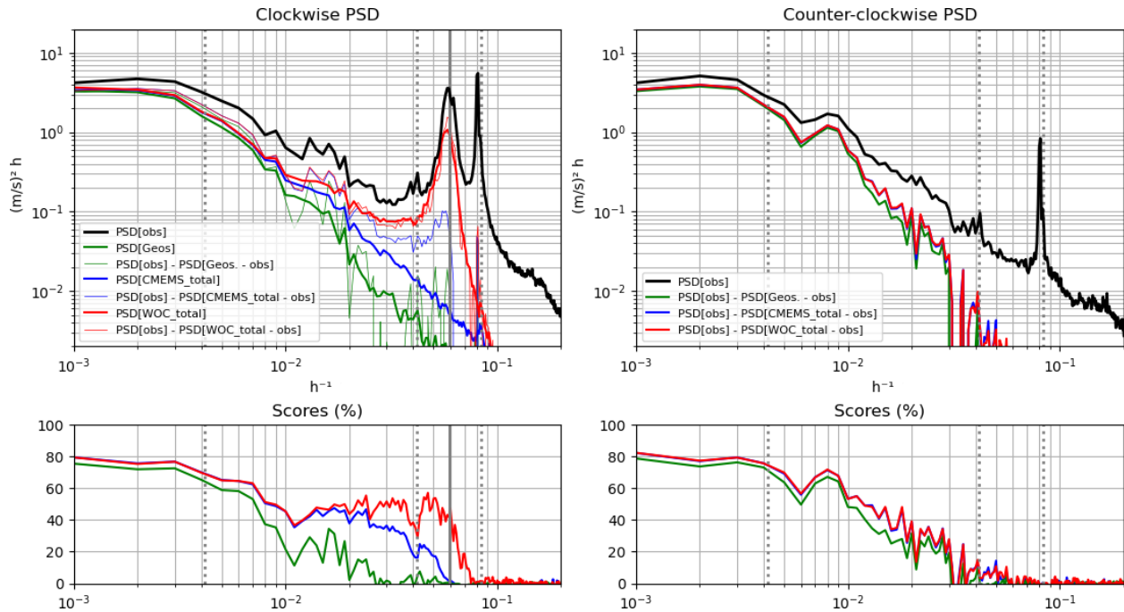
Figure 4. Upper-left panel: power spectral density (in the clockwise time-frequency domain between 1000 and 2 h) of the drogued-drifter current observations in the 40 to 50° N latitude range, in black. The thick-colored curves represent the power spectral densities of the various estimates (geostrophy, CMEMS MOB-TAC and WOC impulse function estimates in green, blue, and red, respectively). The thin-colored curves represent the spectrum of the observations minus the spectra of the difference between the estimation and the observations. Upper-right panel: same, in the counter-clockwise direction. Lower panels: ratio between the thin-colored curves and the black curve of the upper panels, multiplied by 100, representing the percentages of reconstruction (explained variance). The vertical dotted lines indicate the 10 d, 24 and 12 h frequencies, respectively from left to right and the vertical solid line indicates the inertial frequency at 45° N (clockwise only).
