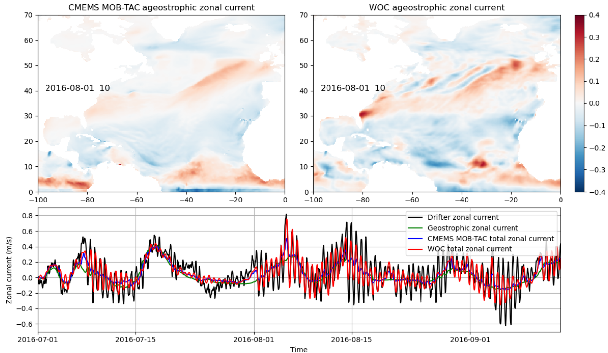
Figure 3. Snapshots of the ageostrophic zonal current from the CMEMS MOB-TAC (upper left) and from the WOC (upper right). Bottom: time series of the total zonal current measured by an independent drifter (black), with a co-location of the geostrophic, CMEMS MOB-TAC total and WOC total zonal current in green, blue and red respectively.
