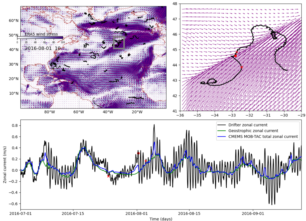
Figure 1. Illustration of the main datasets used in the study. Upper-left panel: a snapshot of the ERA5 wind stress superimposed with the ensemble of drifter positions over \pm 20 d. Upper right: zoom of the first panel highlighting the presence of a drifter near a strong atmospheric front (the red dot is the position at the time of the wind-stress map, the red “x” and “+” 8 d before and 2 d after respectively). Lower panel: time series of the zonal velocities derived from the drifter trajectory (black), with a colocation of the geostrophy (green) and the total surface zonal current from CMEMS-MOB-TAC (blue).
