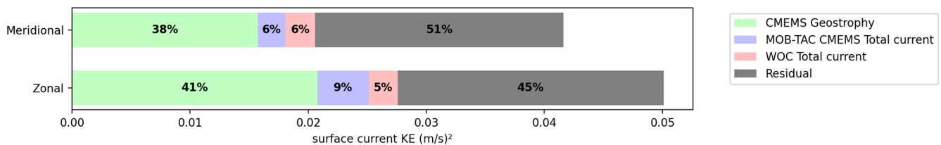
Figure 7. Same as Fig. 6 averaged globally (area weighted).
