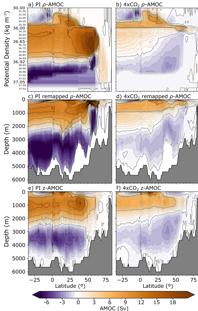
Figure 1. Mean AMOC strength in units of Sverdrup ( 1 \text{ Sv} \equiv 10^6 \text{ m}^3 \text{ s}^{-1} ) averaged over the last 50 years of the PI and 4\times\text{CO}_2 simulations. Panels show (a, b) \rho -AMOC, (c, d) \rho -AMOC remapped into depth coordinates, and (e, f) z -AMOC for (a, c, e) PI and (b, d, f) 4\times\text{CO}_2 . In (c, d), \rho -AMOC is remapped into depth coordinates by loading the mean layer thickness of each density class, cumulatively summing these thicknesses to obtain the bottom depth of each class, then shifting the cumulative sum down one index (with the surface layer reset to zero) so that each transport bin appears at the depth of its upper boundary.
