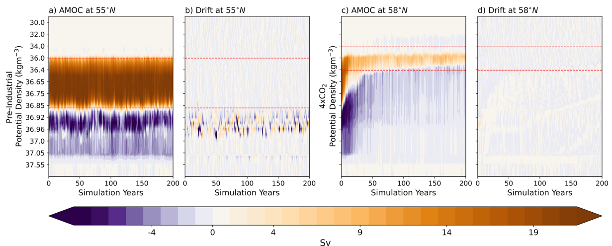
Figure A2. Hovmöller diagrams of \rho -AMOC (a, c) and model drift (b, d) in density space for PI (a, b) and 4xCO 2 (c, d). Red dashed lines denote the upper and lower density bounds of the \rho -AMOC upper limb, computed from the mean over the last 50 years of each simulation. The \rho -AMOC maximum latitude for both simulations is displayed in Table 1.
