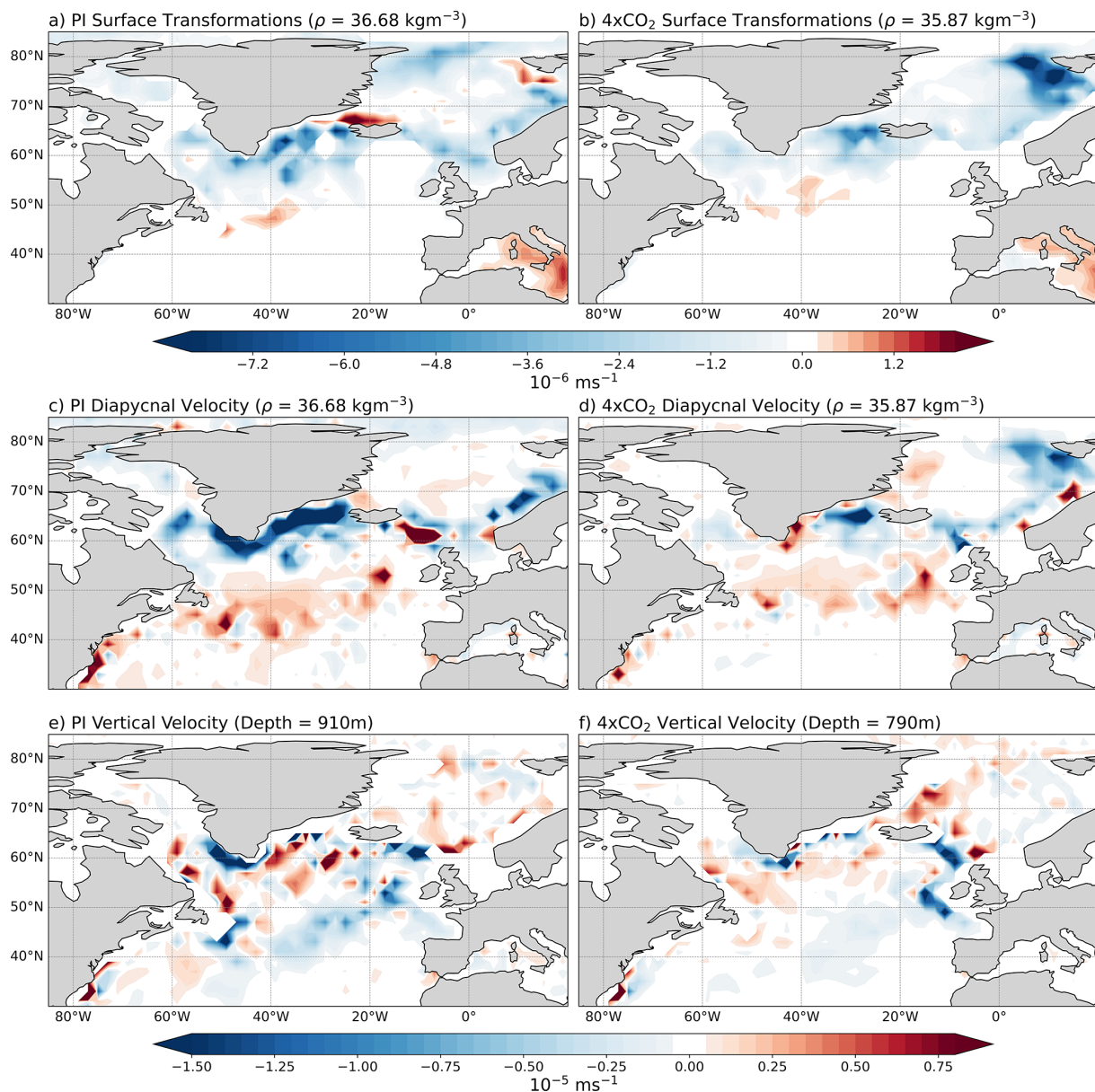
Figure 7. Mean surface-forced diapycnal water mass transformations ( \bar{\psi}_s ; a, b ), diapycnal velocity ( c, d ) and vertical velocity ( e, f ) under ( a, c, e ) PI and ( b, d, f ) 4xCO 2 conditions. Depth and density levels differ: PI (910 m, 36.68 \text{ kg m}^{-3} ) vs. 4xCO 2 (790 m, 35.87 \text{ kg m}^{-3} ). Negative values (blue) indicate downward fluxes (buoyancy loss), whereas positive values (red) indicate upward fluxes (buoyancy gain).
