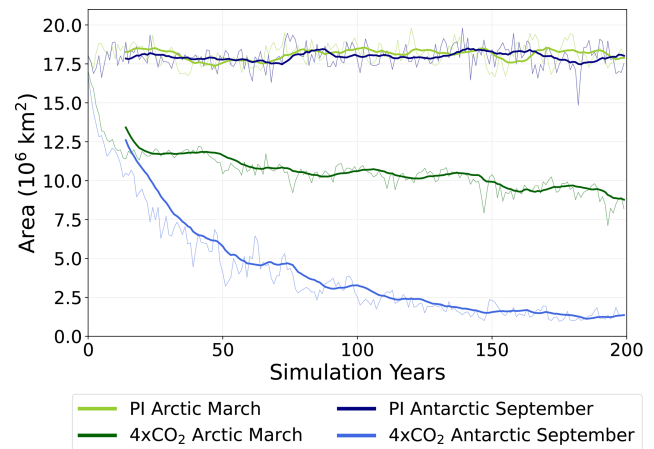
Figure 3. Winter Sea ice area in the Arctic and Southern Oceans in PI and 4xCO 2 simulations. Annual means are represented in thin lines and a superimposed 15 year rolling mean is represented in thick lines to highlight multidecadal variability.
