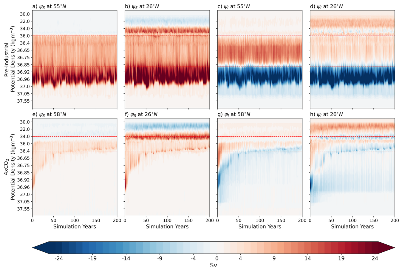
Figure 6. Hovmöller diagrams of surface and interior transformations in density space for PI (a–d) and 4xCO 2 (e–h). First two columns (a, b, e, f) display the surface transformations, \psi_S , at (a, e) the \rho -AMOC maximum latitude and (b, f) 26°N, while last two columns (c, d, g, h) display the interior transformations, \psi_I , at (c, g) the \rho -AMOC maximum latitude and (d, h) 26°N. Positive (red) values indicate transformations toward lighter waters (buoyancy gain/upwelling), and negative (blue) values indicate transformations toward denser waters (buoyancy loss/downwelling). Red dashed lines denote the upper and lower density bounds of the \rho -AMOC upper limb, computed from the mean over the last 50 years of each simulation. The \rho -AMOC maximum latitude for both simulations is displayed in Table 1.
