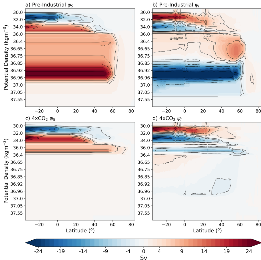
Figure 4. Mean surface ( \psi_S ; a, c ) and interior ( \psi_I ; b, d ) water mass transformation streamfunctions in (a, b) PI and (c, d) 4xCO 2 , respectively. Blue contours indicate upwelling (i.e., transformations toward lighter waters), while red contours indicate downwelling (i.e., transformations toward denser waters).
