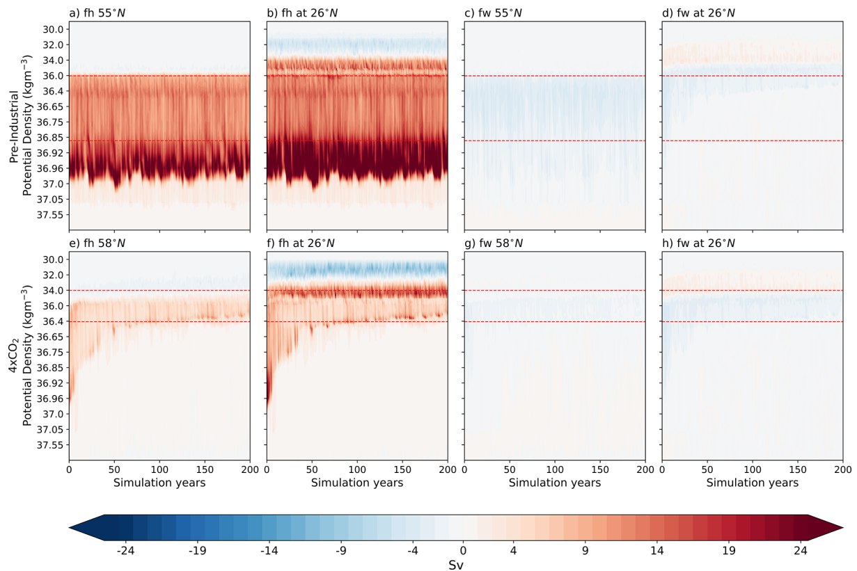
Figure A1. Hovmöller diagrams of the contributions of heat fluxes (FH) and freshwater fluxes (FW) to surface transformations for PI (a–d) and 4xCO 2 (e–h). First two columns (a, b, e, f) display the FH at (a, e) the \rho -AMOC maximum latitude and (b, f) 26°N, while last two columns (c, d, g, h) display the FW at (c, g) the \rho -AMOC maximum latitude and (d, h) 26°N. Positive (red) values indicate transformations toward lighter waters (buoyancy gain/upwelling), and negative (blue) values indicate transformations toward denser waters (buoyancy loss/downwelling). Red dashed lines denote the upper and lower density bounds of the \rho -AMOC upper limb, computed from the mean over the last 50 years of each simulation. The \rho -AMOC maximum latitude for both simulations is displayed in Table 1.
