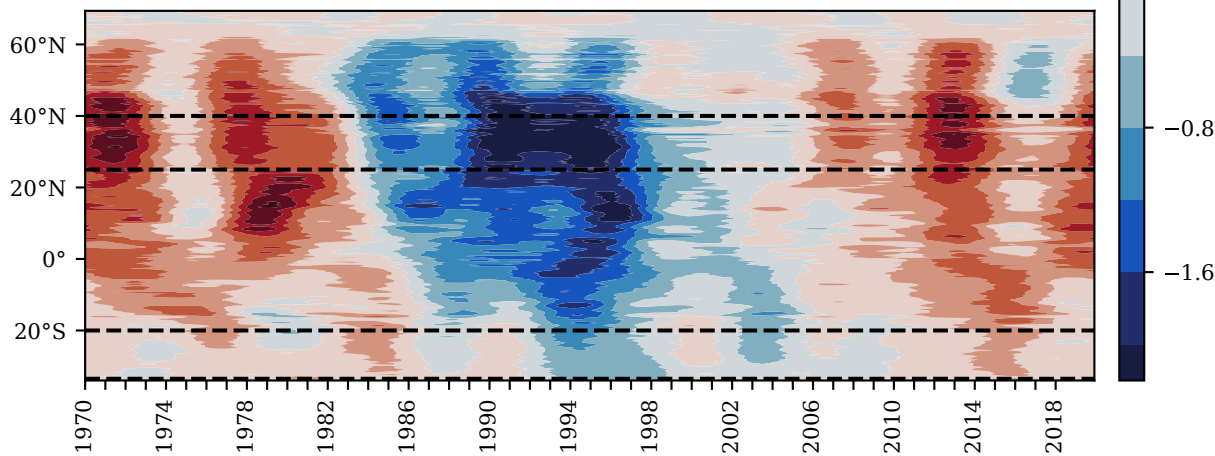
(b) 5 year low-pass filtered
