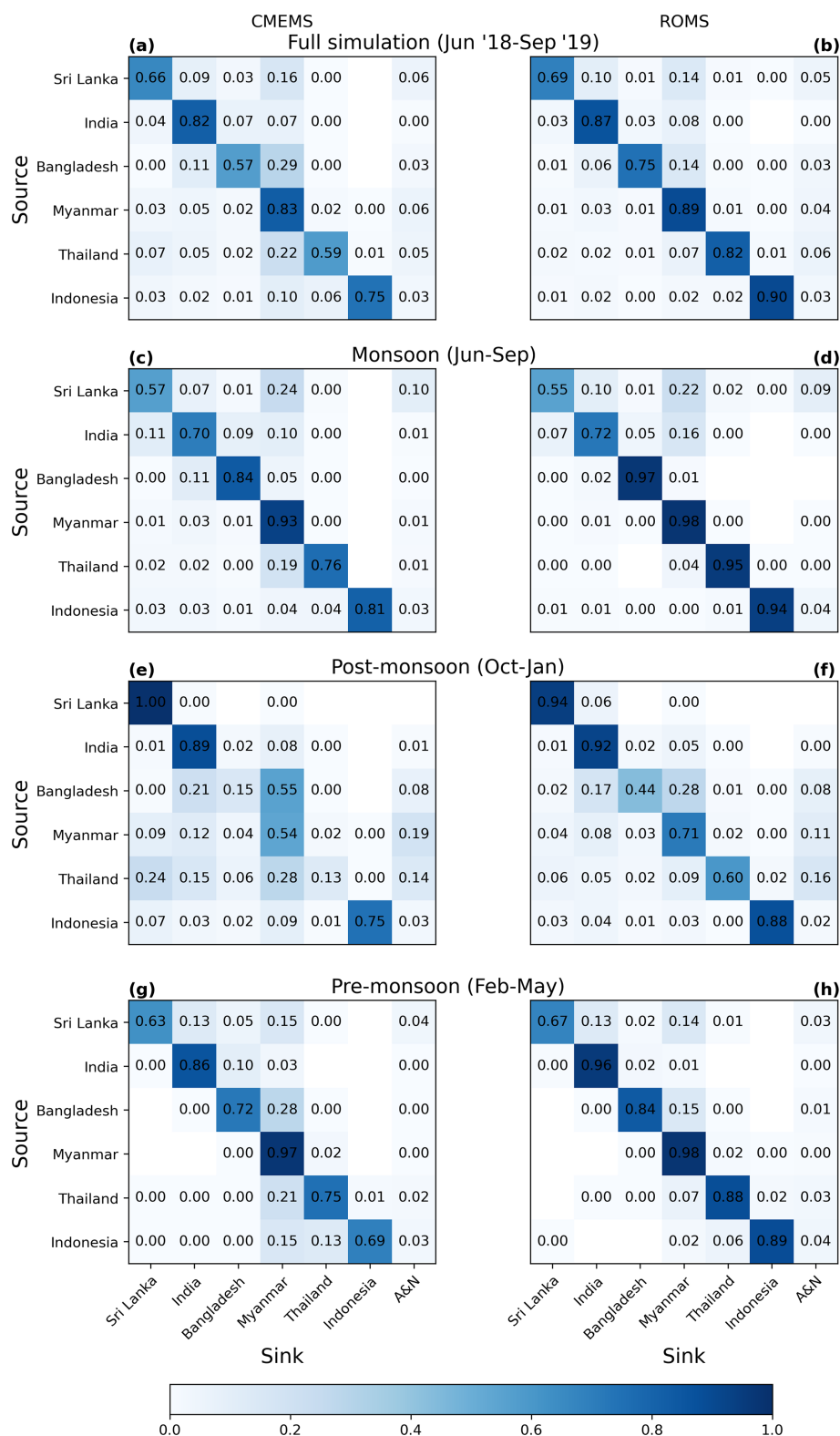
Figure 3. Connectivity matrices showing sources and sinks of particles normalised by the number of particles released from each country. Left column (a, c, e, g) shows results from the CMEMS simulations and the right column (b, d, f, h) shows those of the ROMS runs. Top row shows connectivity over the course of the full simulation (a, b); second row shows results from particles released during the monsoon season (June–September 2018; c, d); third row shows connectivity of particles released during the post-monsoon season (October 2018–January 2019; e, f); and the bottom row shows results of particles released in the pre-monsoon season (February–May 2019; g, h). Blank boxes show where no particles have connected between countries; boxes showing “0.0” have been rounded down but are in fact a non-zero value.
