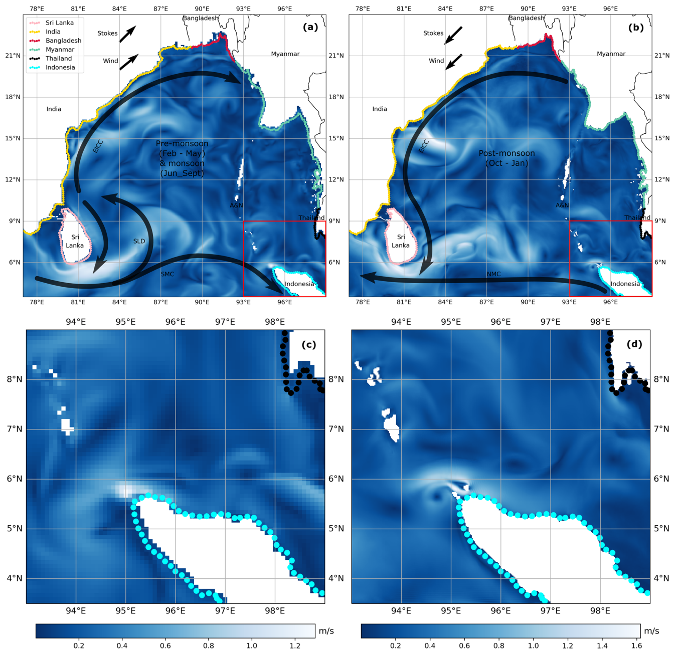
Figure 1. Major currents in the Bay of Bengal during the pre-monsoon (February–May) and monsoon seasons (June–September) (a) and the post-monsoon season (October–January) (b). EICC is East India Coastal Current; SLD is Sri Lanka Dome; SMC is Southwest Monsoon Current; NMC is Northeast Monsoon Current; A&N is Andaman and Nicobar Islands. Arrows of Stokes drift and wind velocities show the mean direction averaged over each time period; magnitudes are arbitrary. Blue backgrounds show ocean current speeds on 24 July 2018 from the CMEMS model (a) and ROMS model (b) and areas in the red box are enlarged in (c) and (d), respectively. Coloured markers indicate particle release locations and are colour-coded by country of origin.
