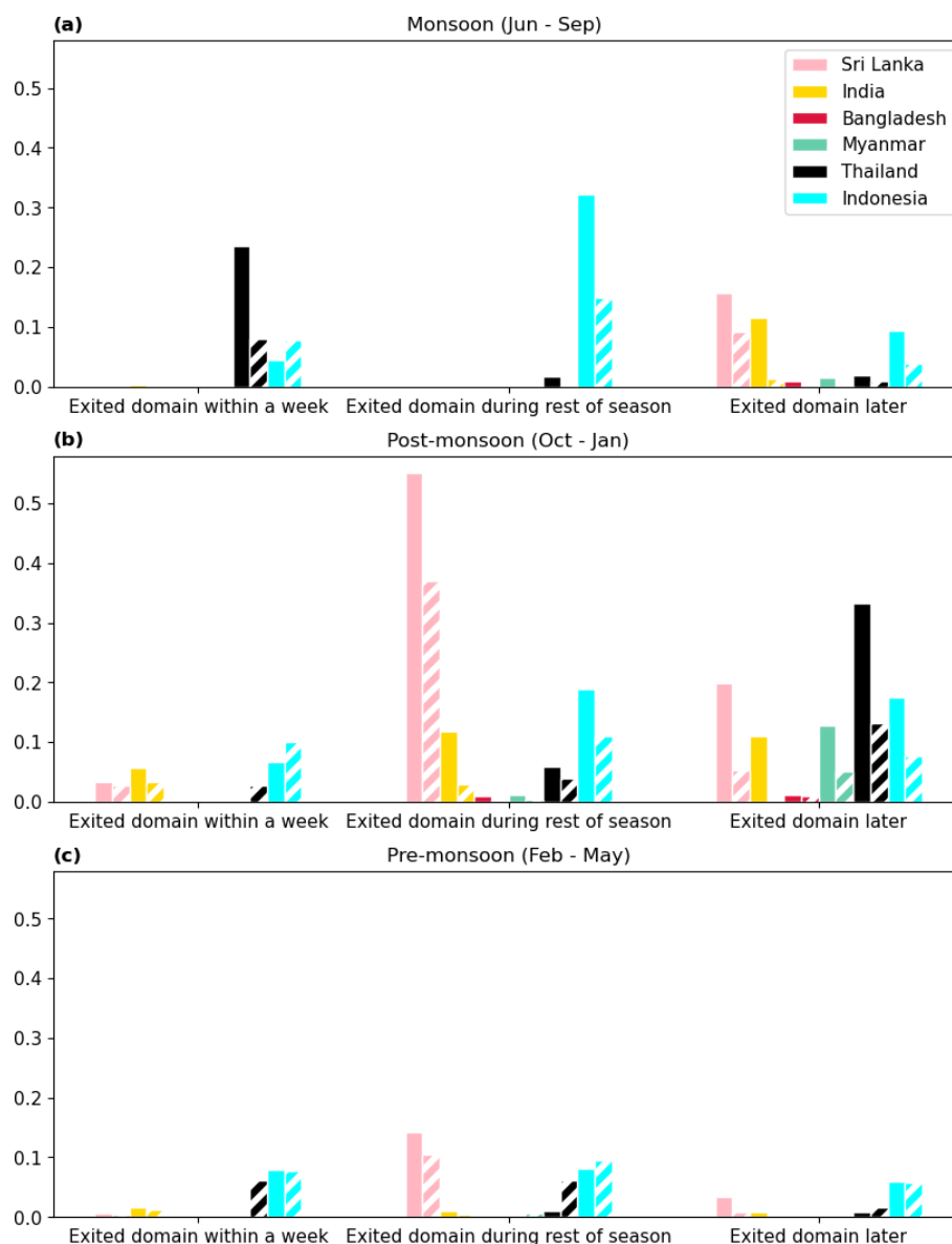
Figure 6. Fraction of particles released during the monsoon season (a), post-monsoon season (b) and pre-monsoon season (c) from each country that left the domain within given time frames. Bars are colour-coded by country with solid bars representing CMEMS particles and striped bars representing ROMS.
