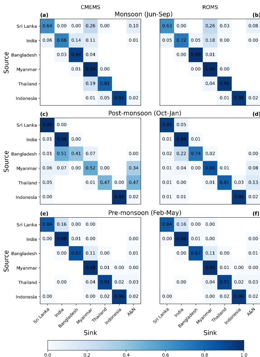
Figure 4. Connectivity between source and sink locations made by particles that were released AND beached during the specified period of time: monsoon period only (June–September 2018; a, b ), post-monsoon season only (October 2018–January 2019; c, d ), and pre-monsoon season only (February–May 2019; e, f ). Results from the CMEMS run are shown in the left panel ( a, c, e ) and the ROMS run on the right ( b, d, f ). Blank boxes show where no particles have connected between countries; boxes showing “0.0” have been rounded down but are in fact a non-zero value.
