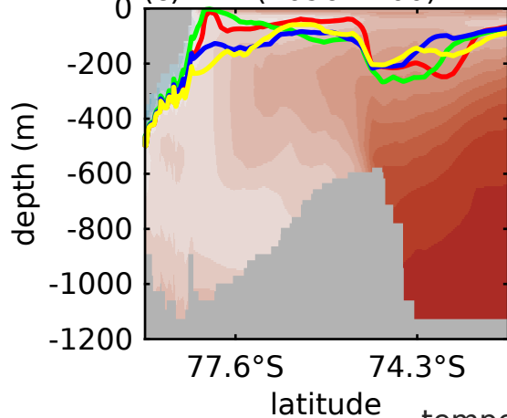
(c) REF (2096-2100)
