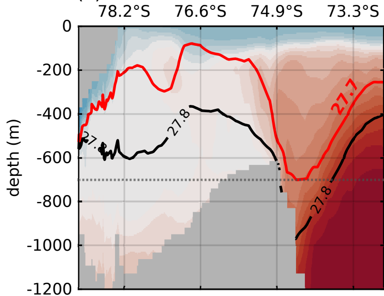
(c) summer
