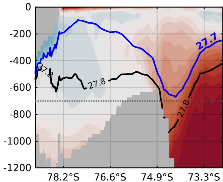
(c) summer
