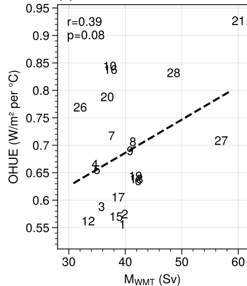
(e) M_{WMT} vs. OHUE
