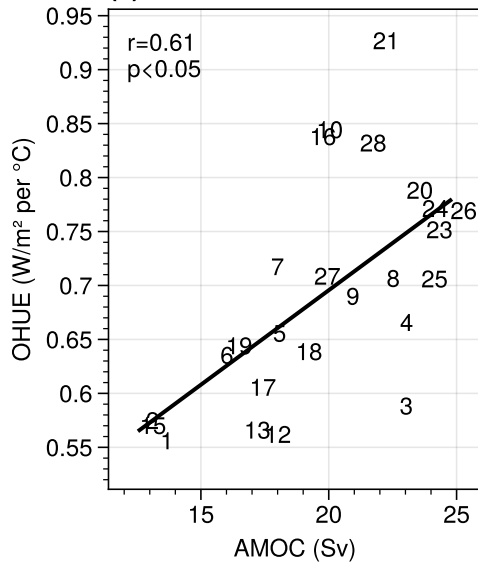
(c) AMOC vs. OHUE
