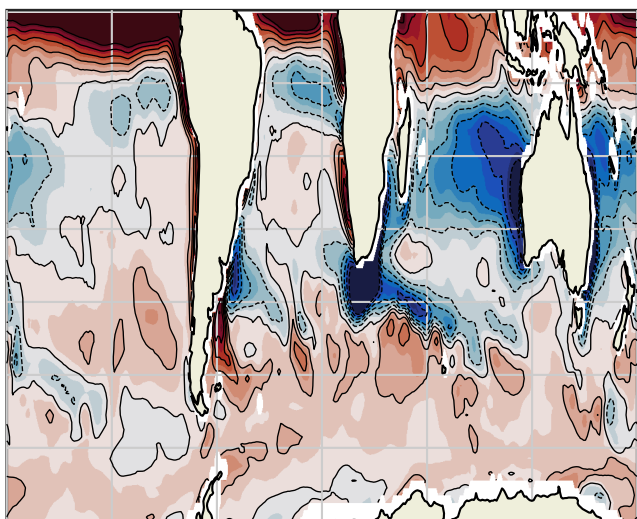
(f) B^{\text{surf}} ECCO
