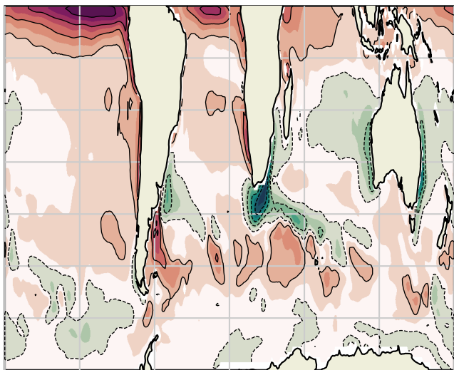
(c) Q_{\text{tot}} ECCO
