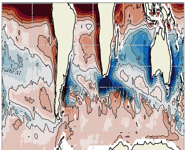
(e) B^{\text{surf}} OAflux adjusted
