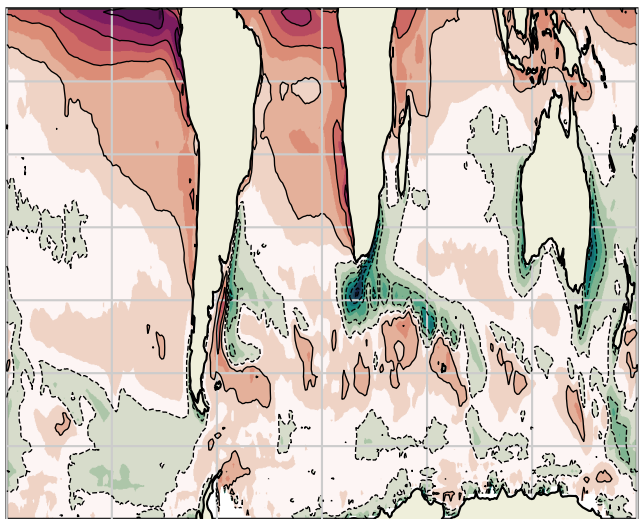
(b) Q_{\text{tot}} OAflux adjusted
