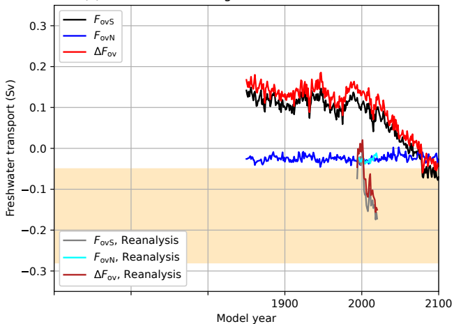
(c) Freshwater convergence, HR-CESM, Hist/RCP8.5
