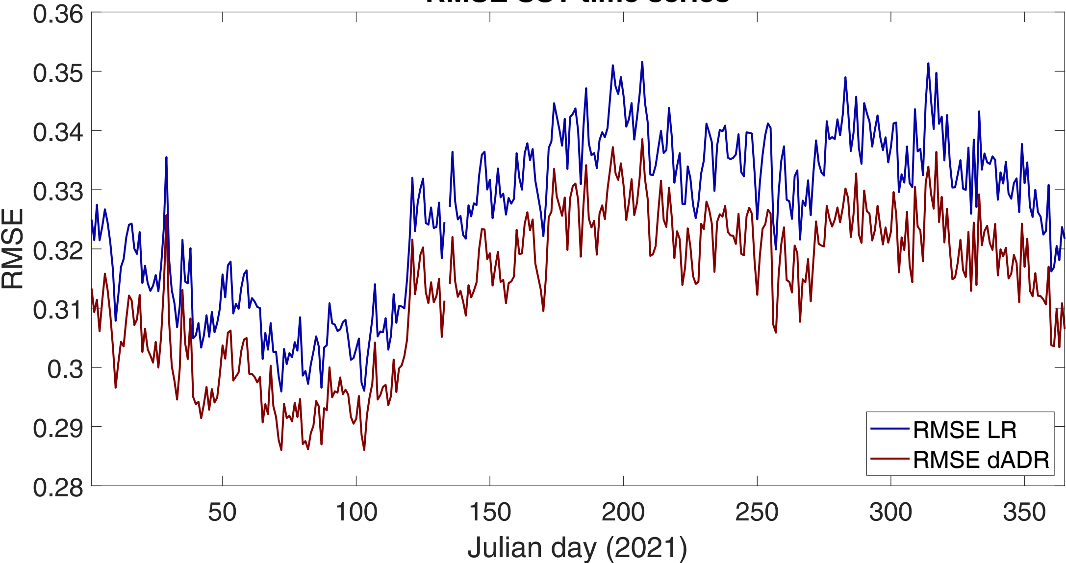
RMSE SST time series
