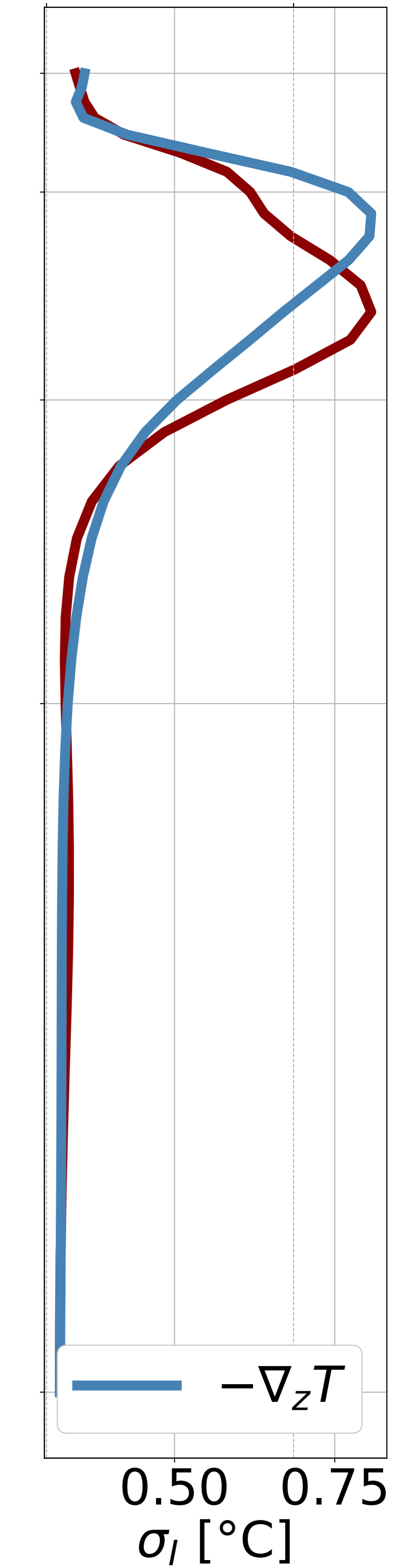
(c) EMed -\nabla_z T [ ^{\circ}\text{Cm}^{-1} ] 0.0 0.2
