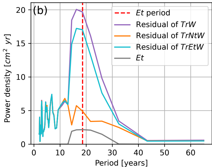
Multitaper spectra
