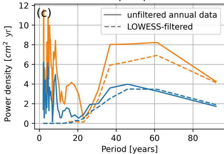
Multitaper spectra
