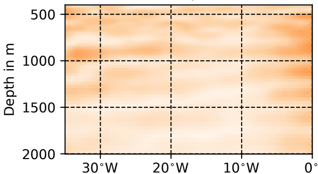
Kelvin wave amplitude
