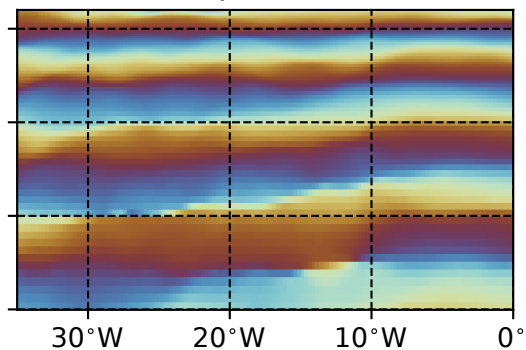
Kelvin wave phase
