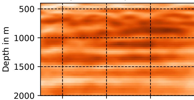
Kelvin wave amplitude
