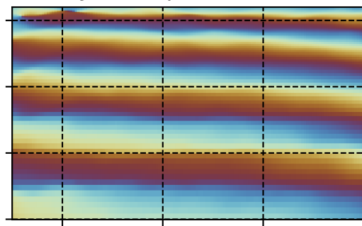
Rossby wave phase
