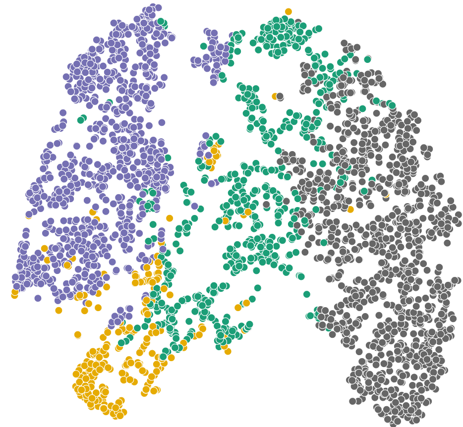
Perplexity 50
