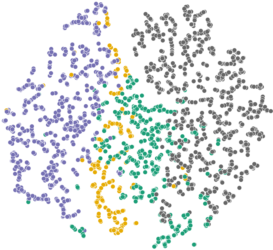
Perplexity 5
