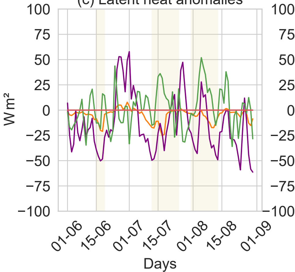
(c) Latent heat anomalies
