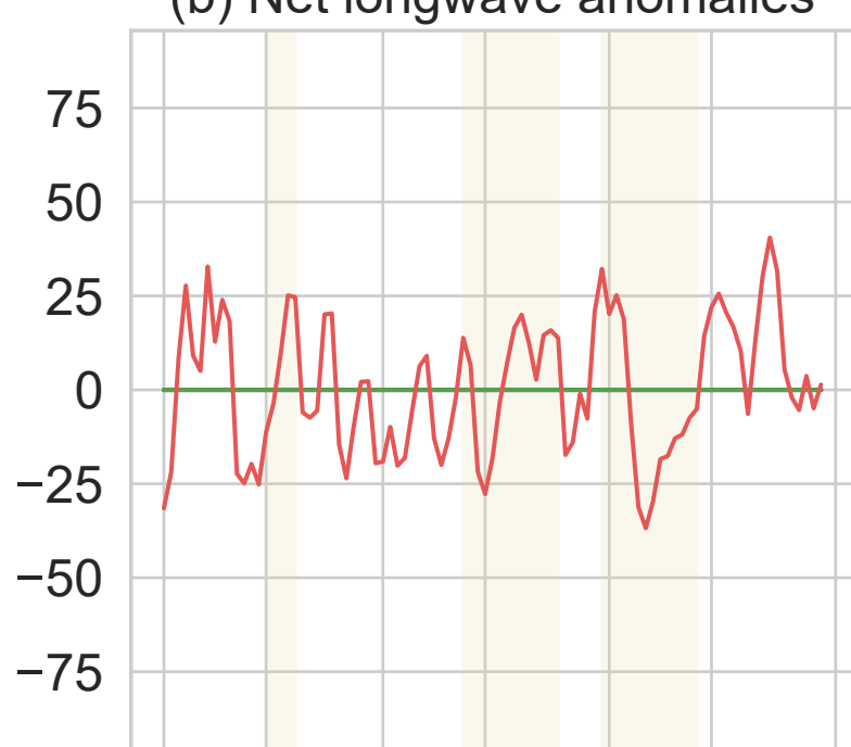
(b) Net longwave anomalies
