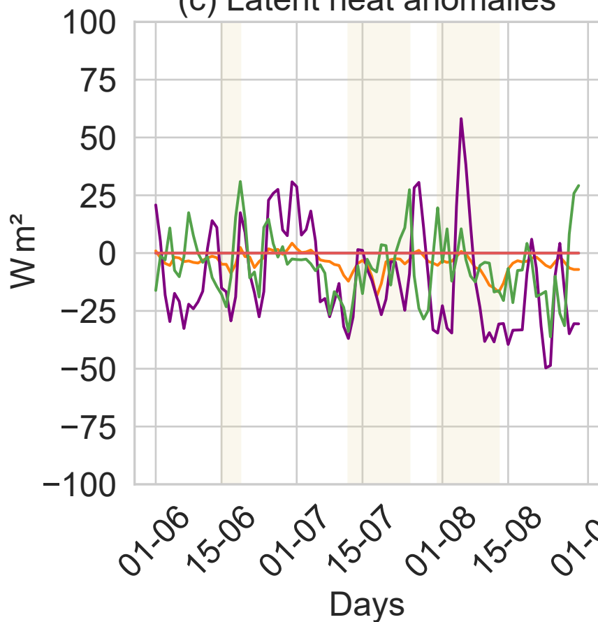
(c) Latent heat anomalies
