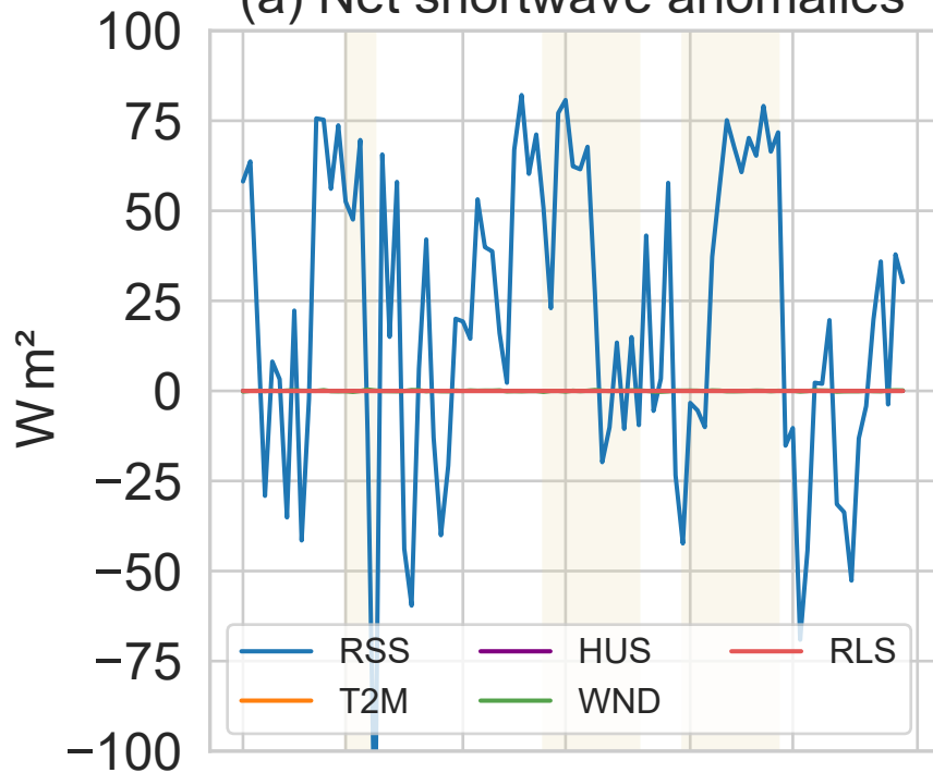
(a) Net shortwave anomalies
