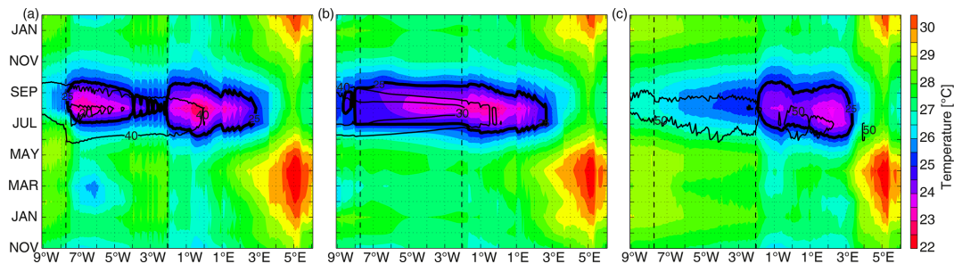
Figure 8. Hovmöller diagrams of SST (°C) along the coast of the GGUS from 9° W to 6° E of (a) the reference experiment and of the idealized experiments (b) without capes and (c) without inertial terms. The thermocline depth (20 °C isotherm) is superimposed (thin contour lines; unit is m). The vertical dashed black lines represent the longitude of Cape Palmas and Cape Three Points – see Fig. 7. The time axis in months extends from November to February of the following year. The 25 °C isotherm is additionally marked to highlight the coastal upwelling (thick contour lines). Model output is taken from Djakouré et al. (2014, 2017).
