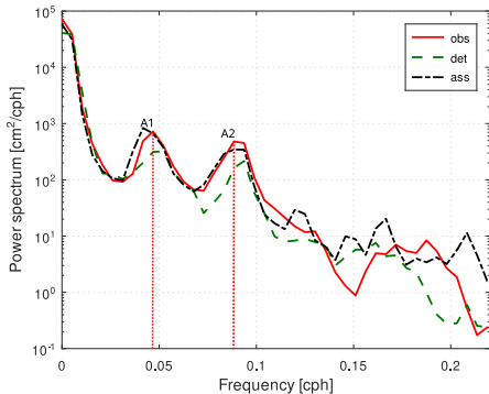
Bari - Power spectral density
