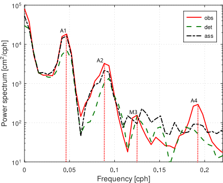
Trieste - Power spectral density
