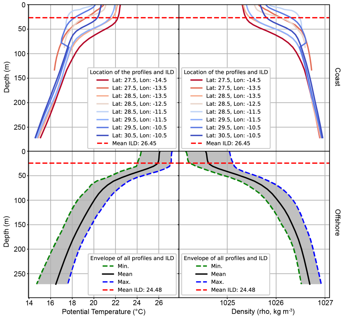
Supplementary figure: Example of a depth-profile (September 1995) of density and temperature at different latitudes for the coastal and offshore area. For the offshore area, minimum, maximum, and mean values of all profiles have been calculated and plotted in an envelope
