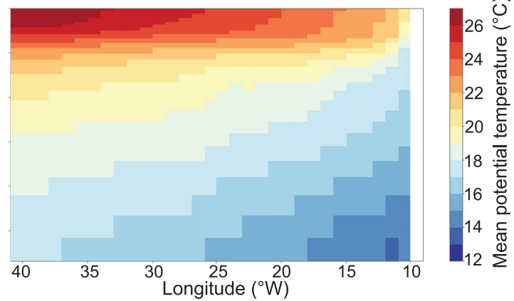
(b) UI_{SST} ( 30.5^{\circ}N )
