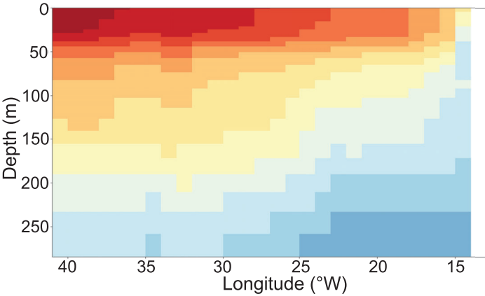
(a) UI_{SST} ( 26.5^{\circ}N )
