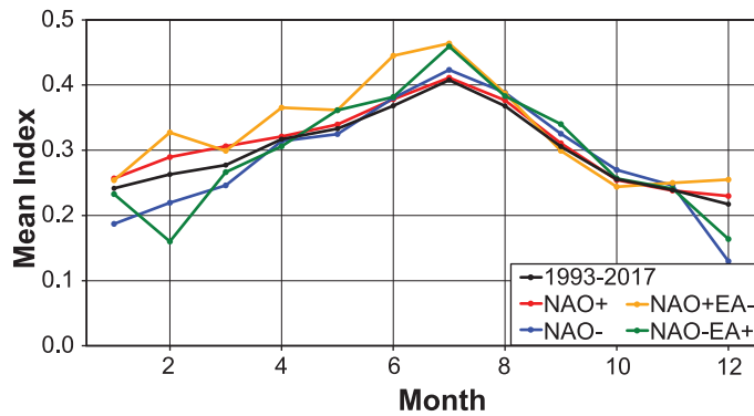
(c) Monthly climatologies of UI_{PFEL}
