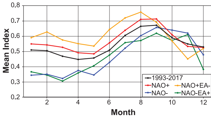
(b) Monthly climatologies of UI_{SST}
